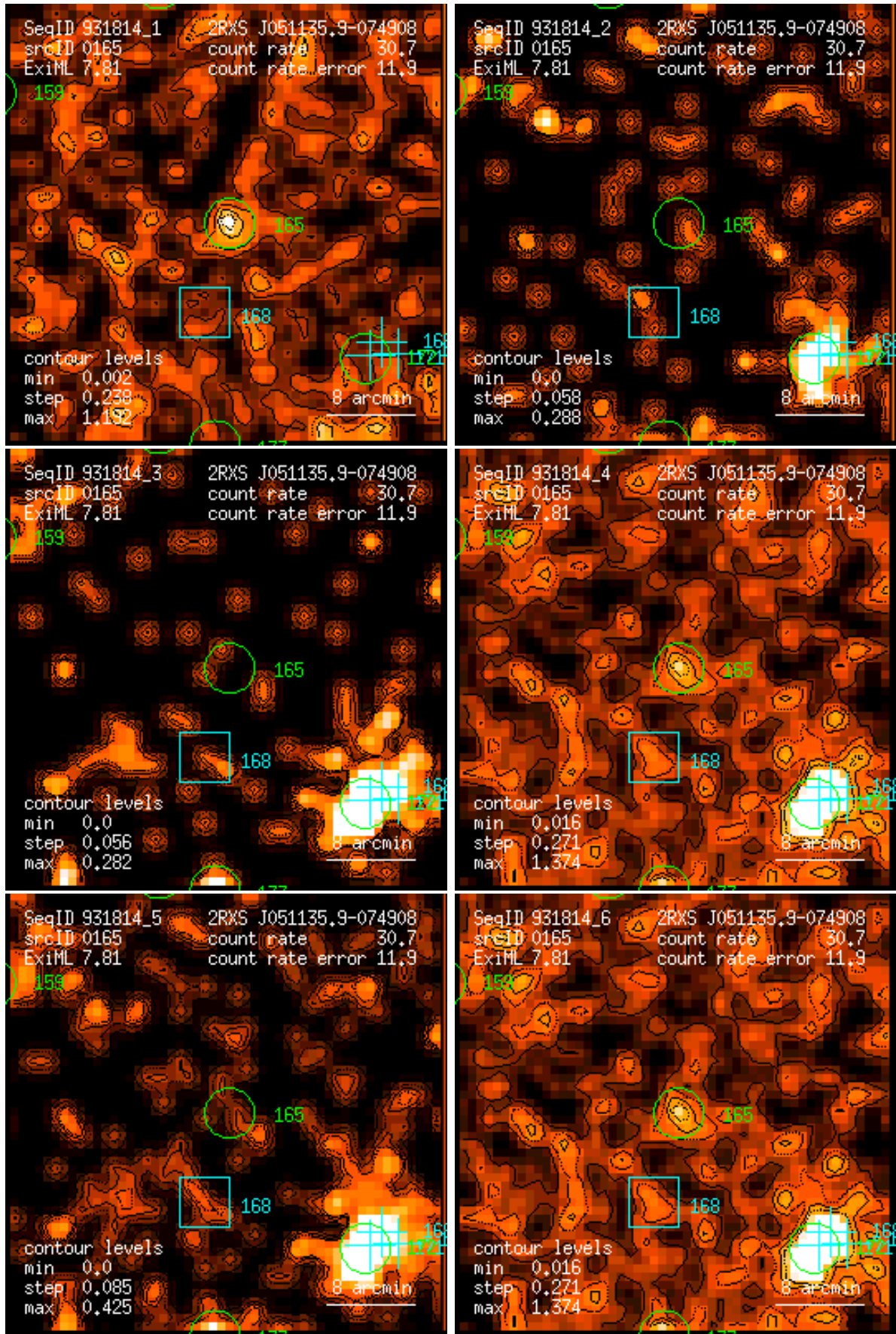
Figure 165: RASS 931814: detection 0165: band rate images, Gaussian filter: (1) PSPC channels 11 – 41, (2) 52 – 90, (3) 91 – 201, (4) 11 – 235, (5) 52 – 201, (6) 11 – 201. Broad band rates in counts/ks. Band rate contour levels in counts/ks/arcmin 2 .
