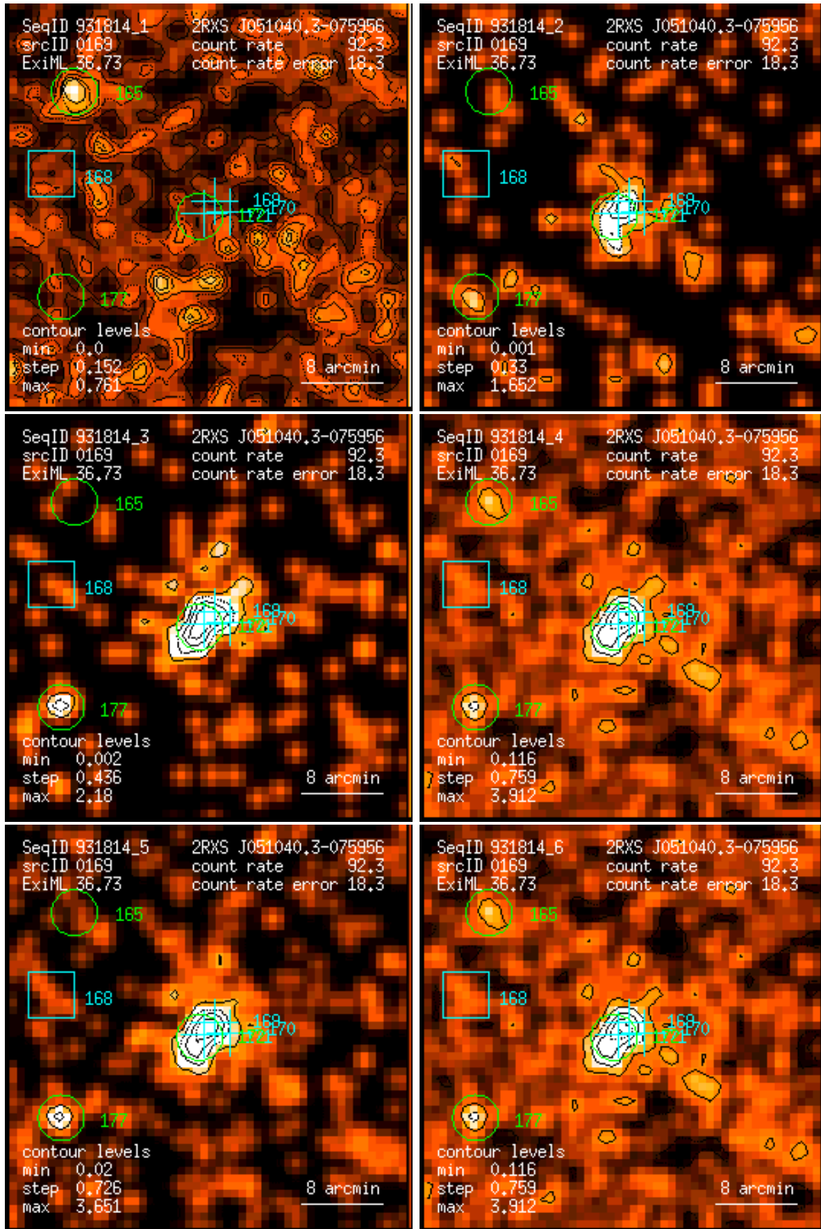
Figure 169: RASS 931814: detection 0169: band rate images, Gaussian filter: (1) PSPC channels 11 – 41, (2) 52 – 90, (3) 91 – 201, (4) 11 – 235, (5) 52 – 201, (6) 11 – 201. Broad band rates in counts/ks. Band rate contour levels in counts/ks/arcmin 2 .
