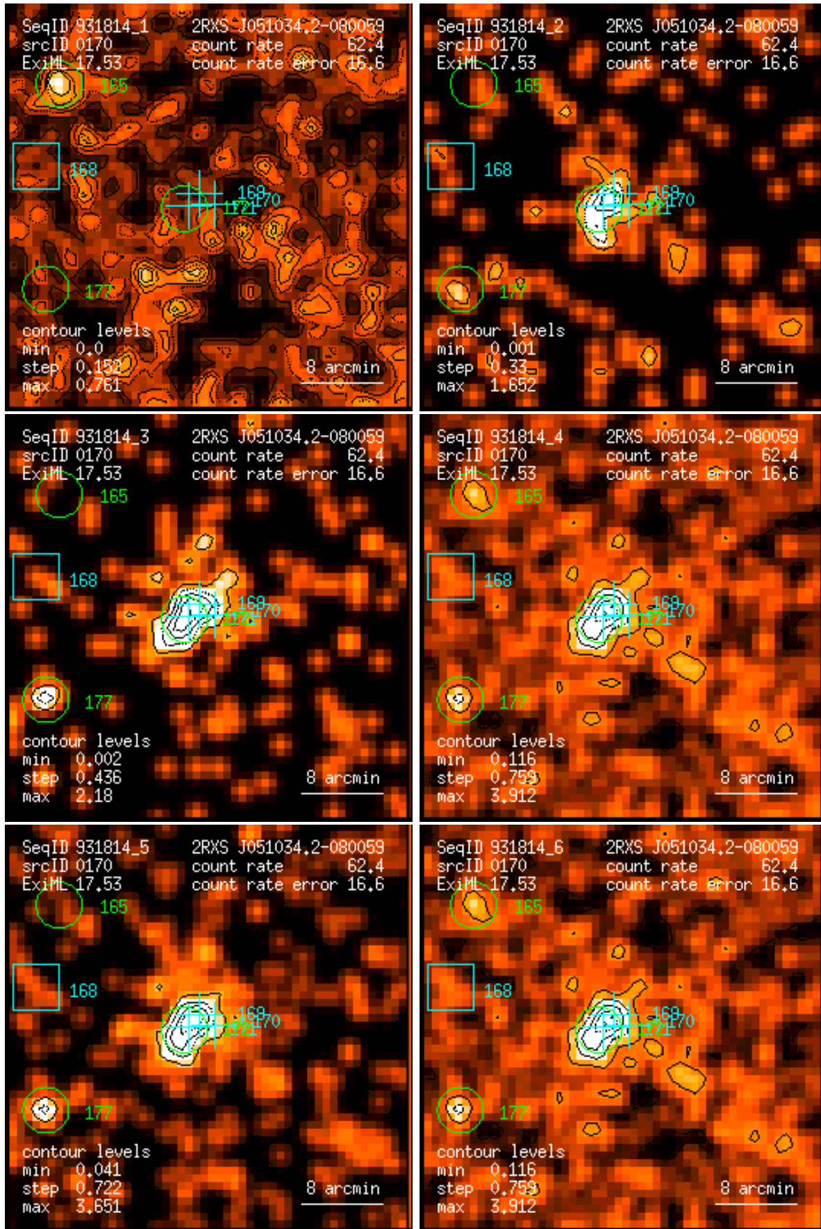
Figure 170: RASS 931814: detection 0170: band rate images, Gaussian filter: (1) PSPC channels 11 – 41, (2) 52 – 90, (3) 91 – 201, (4) 11 – 235, (5) 52 – 201, (6) 11 – 201. Broad band rates in counts/ks. Band rate contour levels in counts/ks/arcmin 2 .
