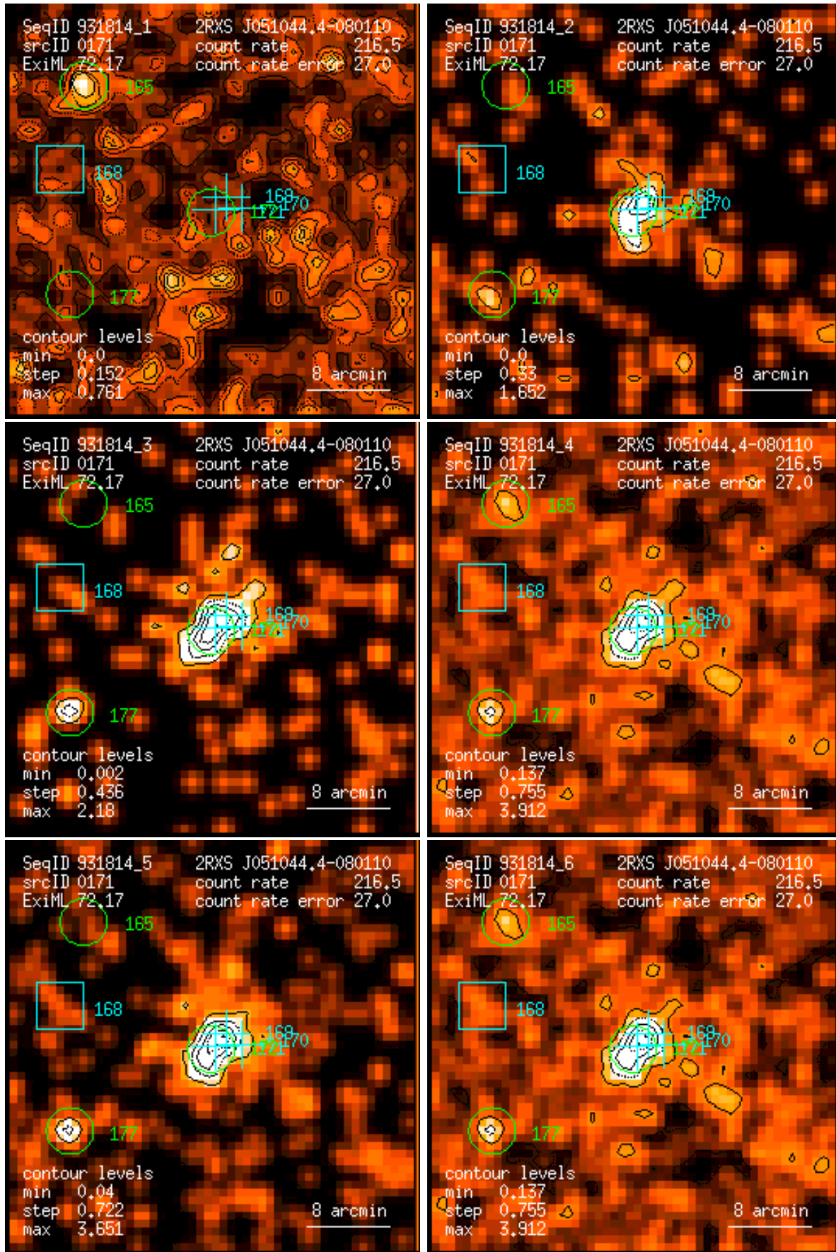
Figure 171: RASS 931814: detection 0171: band rate images, Gaussian filter: (1) PSPC channels 11 – 41, (2) 52 – 90, (3) 91 – 201, (4) 11 – 235, (5) 52 – 201, (6) 11 – 201. Broad band rates in counts/ks. Band rate contour levels in counts/ks/arcmin 2 .
