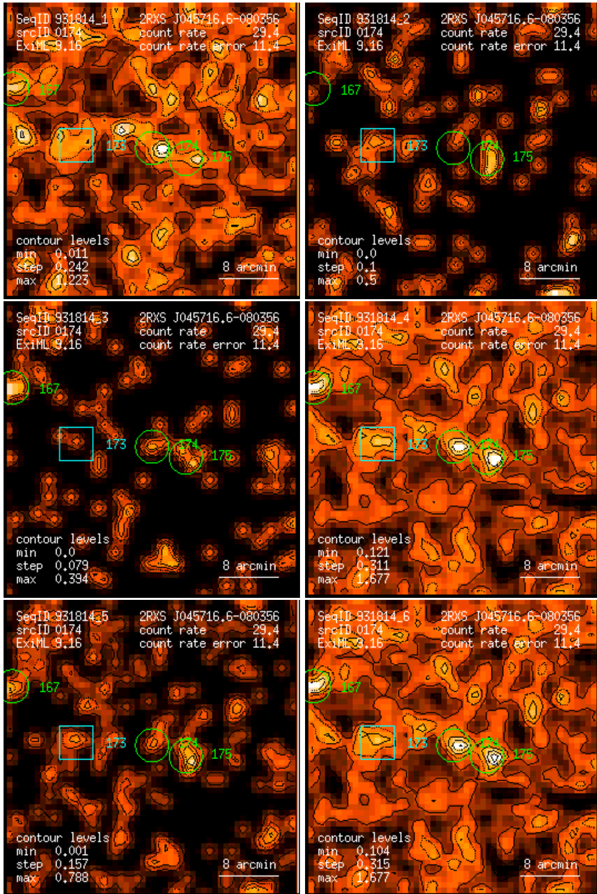
Figure 174: RASS 931814: detection 0174: band rate images, Gaussian filter: (1) PSPC channels 11 – 41, (2) 52 – 90, (3) 91 – 201, (4) 11 – 235, (5) 52 – 201, (6) 11 – 201. Broad band rates in counts/ks. Band rate contour levels in counts/ks/arcmin 2 .
