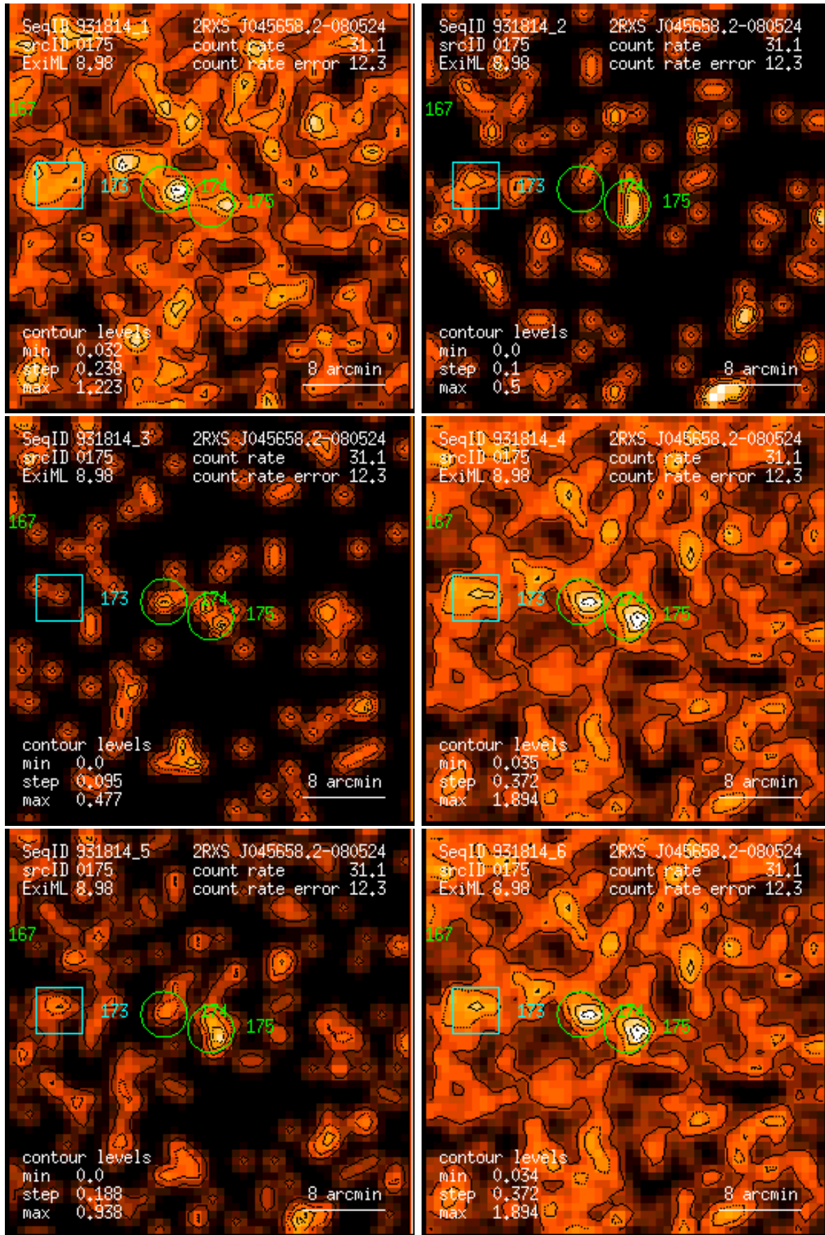
Figure 175: RASS 931814: detection 0175: band rate images, Gaussian filter: (1) PSPC channels 11 – 41, (2) 52 – 90, (3) 91 – 201, (4) 11 – 235, (5) 52 – 201, (6) 11 – 201. Broad band rates in counts/ks. Band rate contour levels in counts/ks/arcmin 2 .
