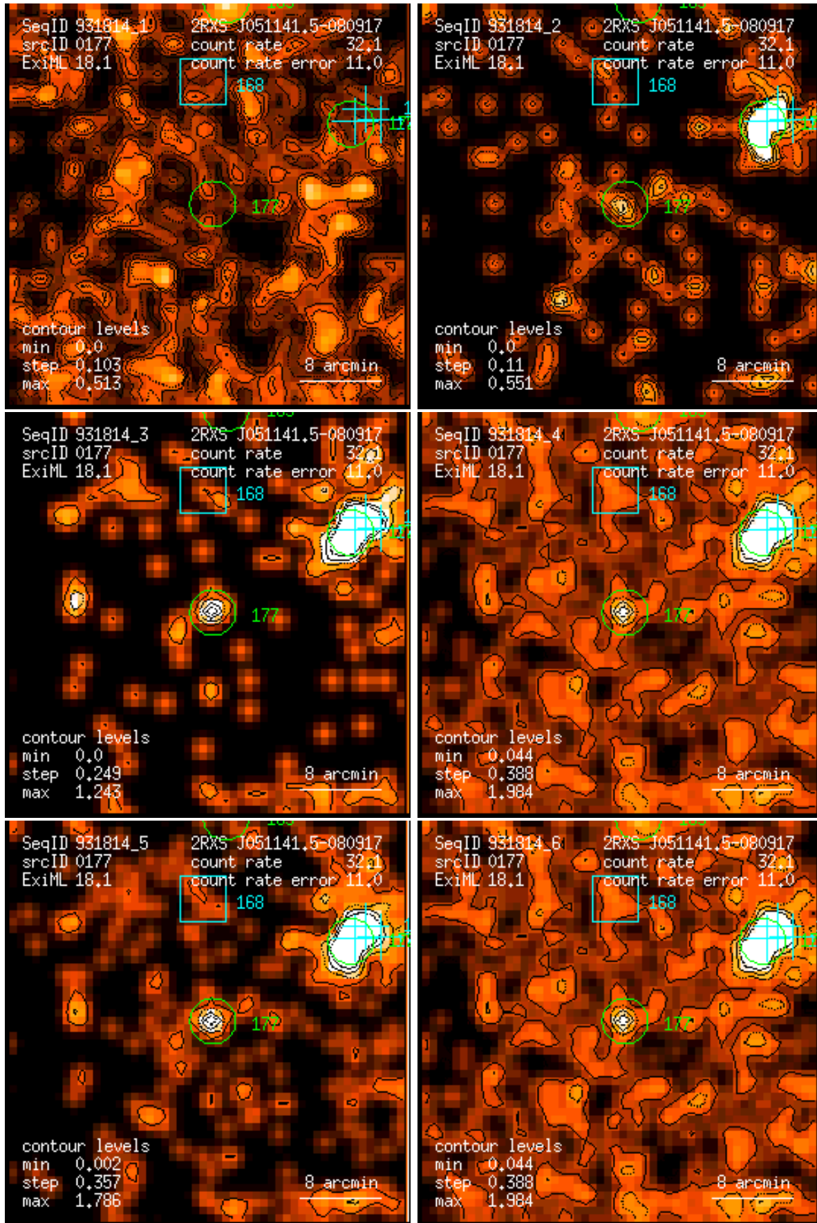
Figure 177: RASS 931814: detection 0177: band rate images, Gaussian filter: (1) PSPC channels 11 – 41, (2) 52 – 90, (3) 91 – 201, (4) 11 – 235, (5) 52 – 201, (6) 11 – 201. Broad band rates in counts/ks. Band rate contour levels in counts/ks/arcmin 2 .
