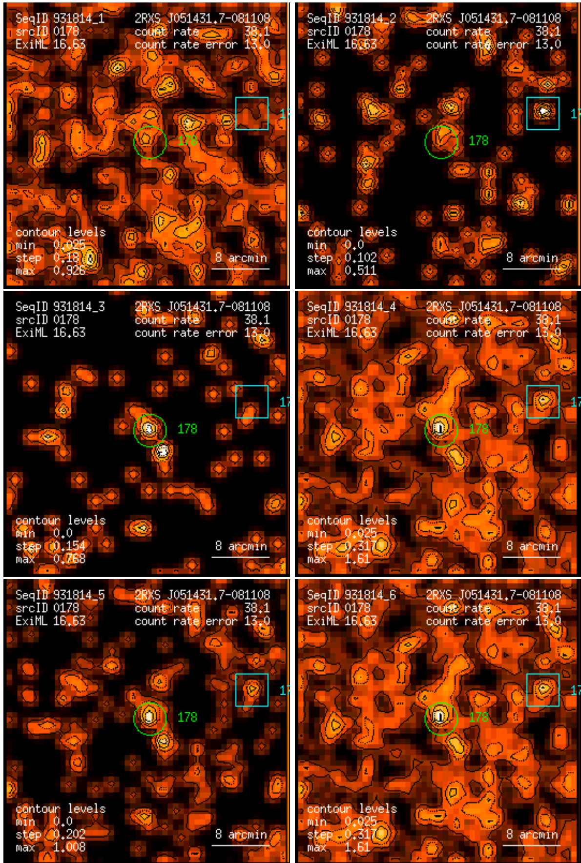
Figure 178: RASS 931814: detection 0178: band rate images, Gaussian filter: (1) PSPC channels 11 – 41, (2) 52 – 90, (3) 91 – 201, (4) 11 – 235, (5) 52 – 201, (6) 11 – 201. Broad band rates in counts/ks. Band rate contour levels in counts/ks/arcmin 2 .
