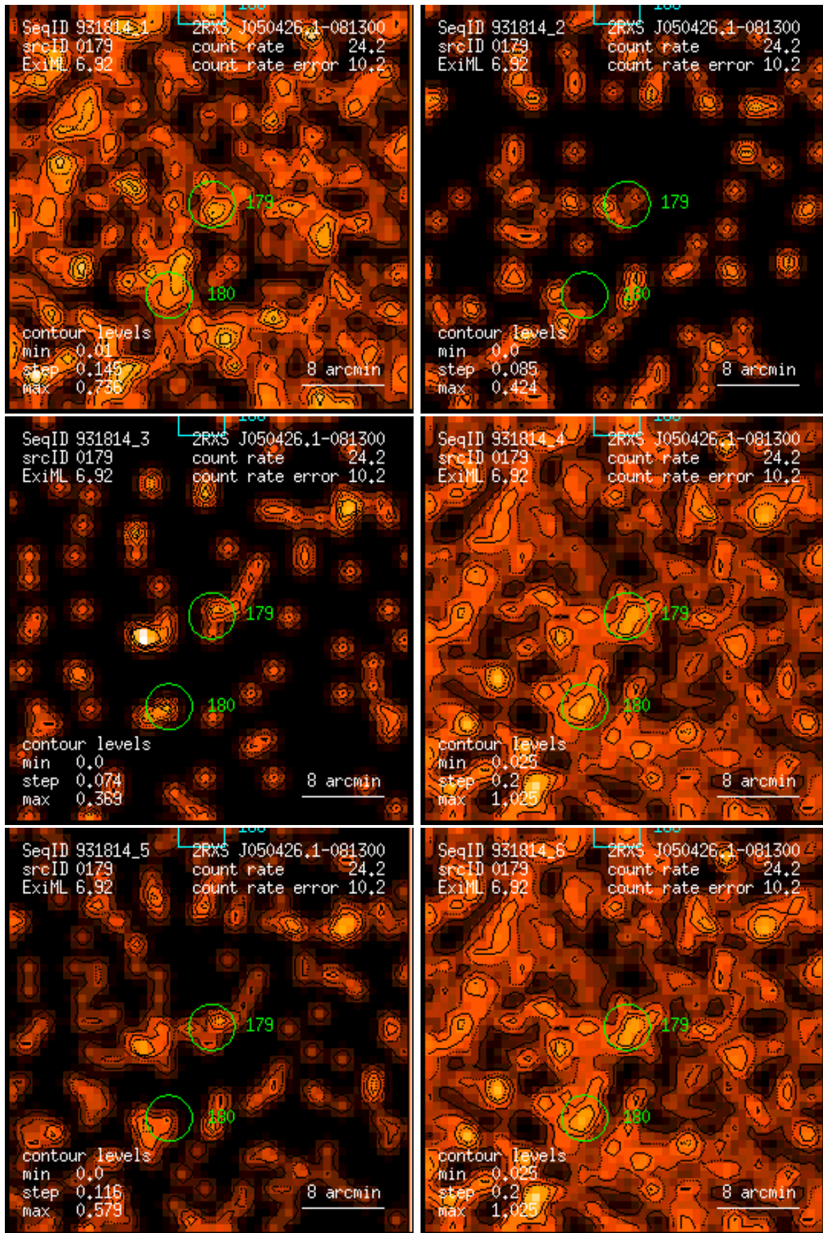
Figure 179: RASS 931814: detection 0179: band rate images, Gaussian filter: (1) PSPC channels 11 – 41, (2) 52 – 90, (3) 91 – 201, (4) 11 – 235, (5) 52 – 201, (6) 11 – 201. Broad band rates in counts/ks. Band rate contour levels in counts/ks/arcmin 2 .
