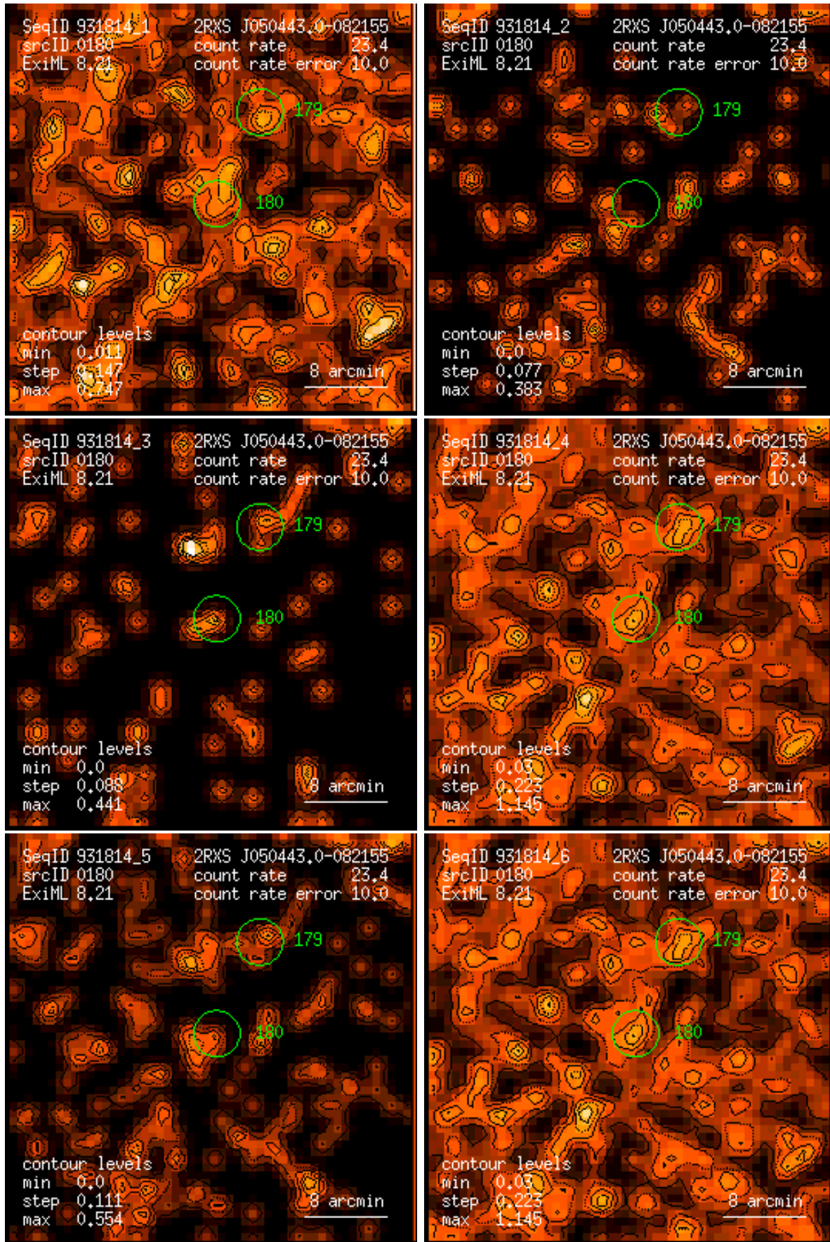
Figure 180: RASS 931814: detection 0180: band rate images, Gaussian filter: (1) PSPC channels 11 – 41, (2) 52 – 90, (3) 91 – 201, (4) 11 – 235, (5) 52 – 201, (6) 11 – 201. Broad band rates in counts/ks. Band rate contour levels in counts/ks/arcmin 2 .
