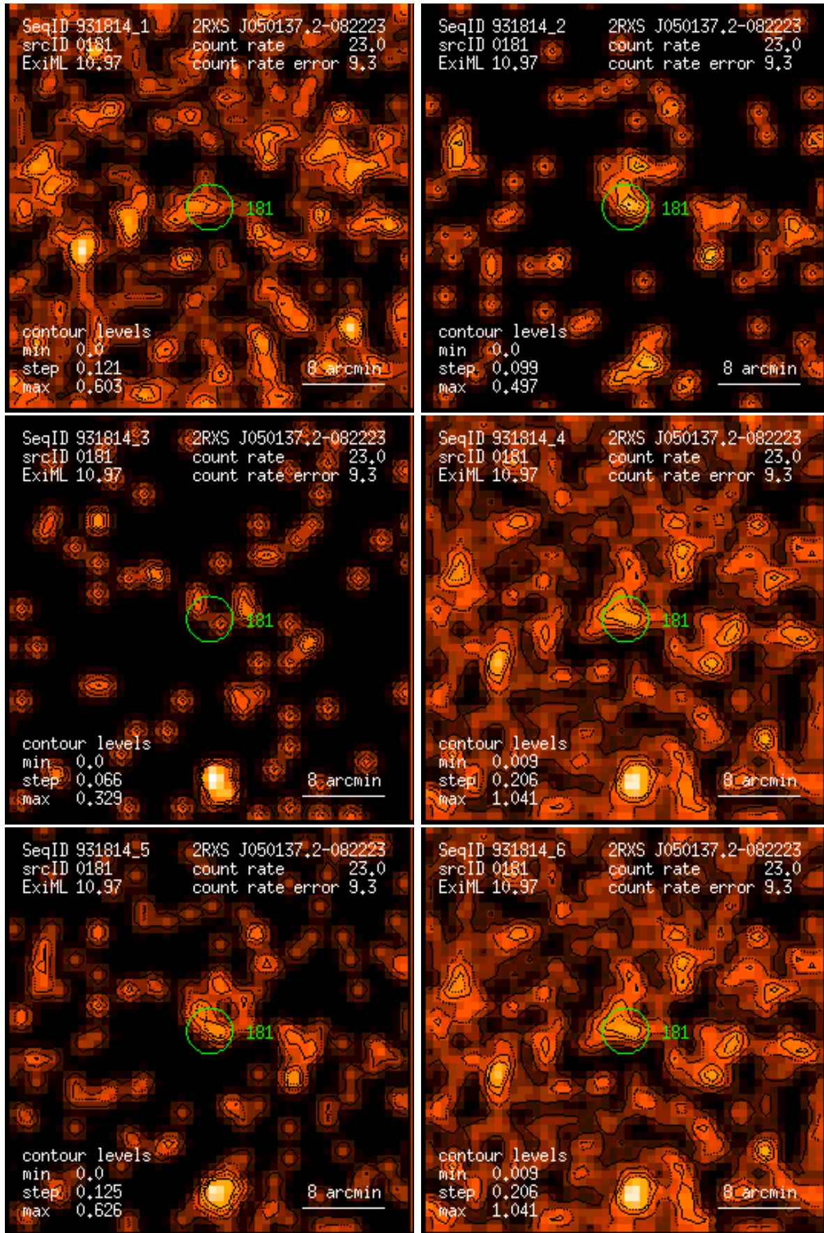
Figure 181: RASS 931814: detection 0181: band rate images, Gaussian filter: (1) PSPC channels 11 – 41, (2) 52 – 90, (3) 91 – 201, (4) 11 – 235, (5) 52 – 201, (6) 11 – 201. Broad band rates in counts/ks. Band rate contour levels in counts/ks/arcmin 2 .
