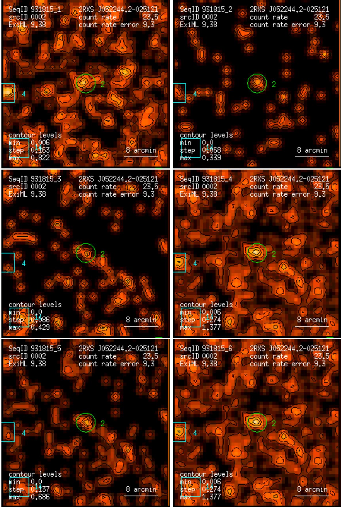
Figure 2: RASS 931815: detection 0002: band rate images, Gaussian filter: (1) PSPC channels 11 – 41, (2) 52 – 90, (3) 91 – 201, (4) 11 – 235, (5) 52 – 201, (6) 11 – 201. Broad band rates in counts/ks. Band rate contour levels in counts/ks/arcmin 2 .
