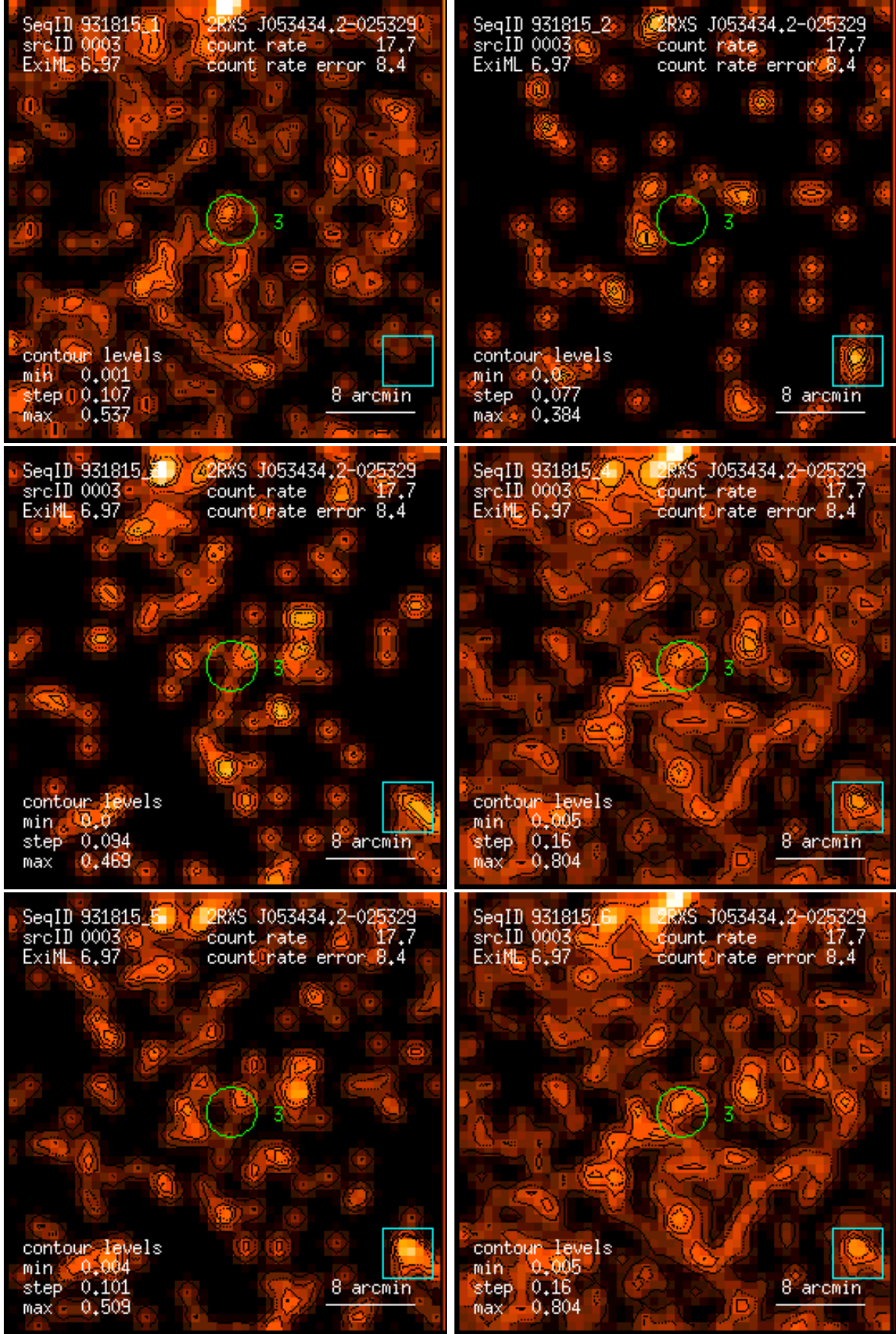
Figure 3: RASS 931815: detection 0003: band rate images, Gaussian filter: (1) PSPC channels 11 – 41, (2) 52 – 90, (3) 91 – 201, (4) 11 – 235, (5) 52 – 201, (6) 11 – 201. Broad band rates in counts/ks. Band rate contour levels in counts/ks/arcmin 2 .
