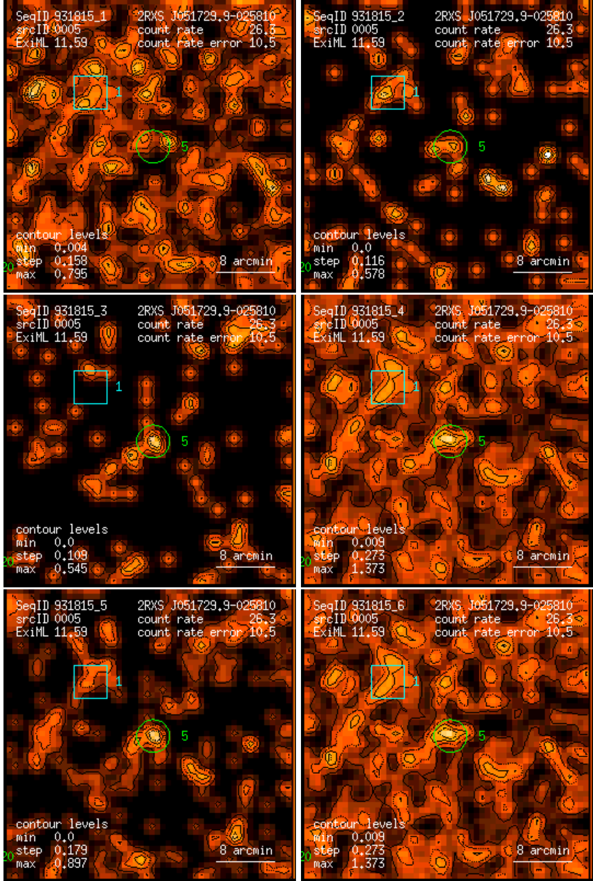
Figure 5: RASS 931815: detection 0005: band rate images, Gaussian filter: (1) PSPC channels 11 – 41, (2) 52 – 90, (3) 91 – 201, (4) 11 – 235, (5) 52 – 201, (6) 11 – 201. Broad band rates in counts/ks. Band rate contour levels in counts/ks/arcmin 2 .
