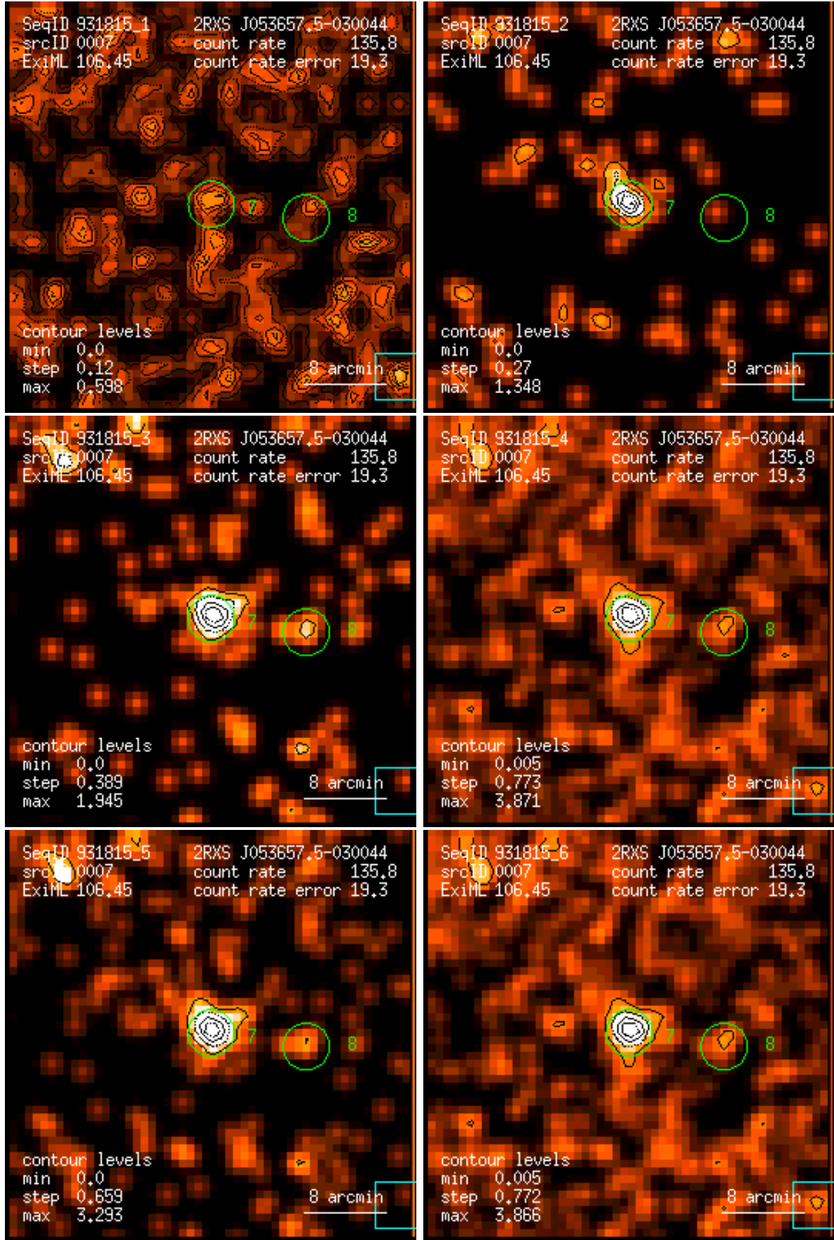
Figure 7: RASS 931815: detection 0007: band rate images, Gaussian filter: (1) PSPC channels 11 – 41, (2) 52 – 90, (3) 91 – 201, (4) 11 – 235, (5) 52 – 201, (6) 11 – 201. Broad band rates in counts/ks. Band rate contour levels in counts/ks/arcmin 2 .
