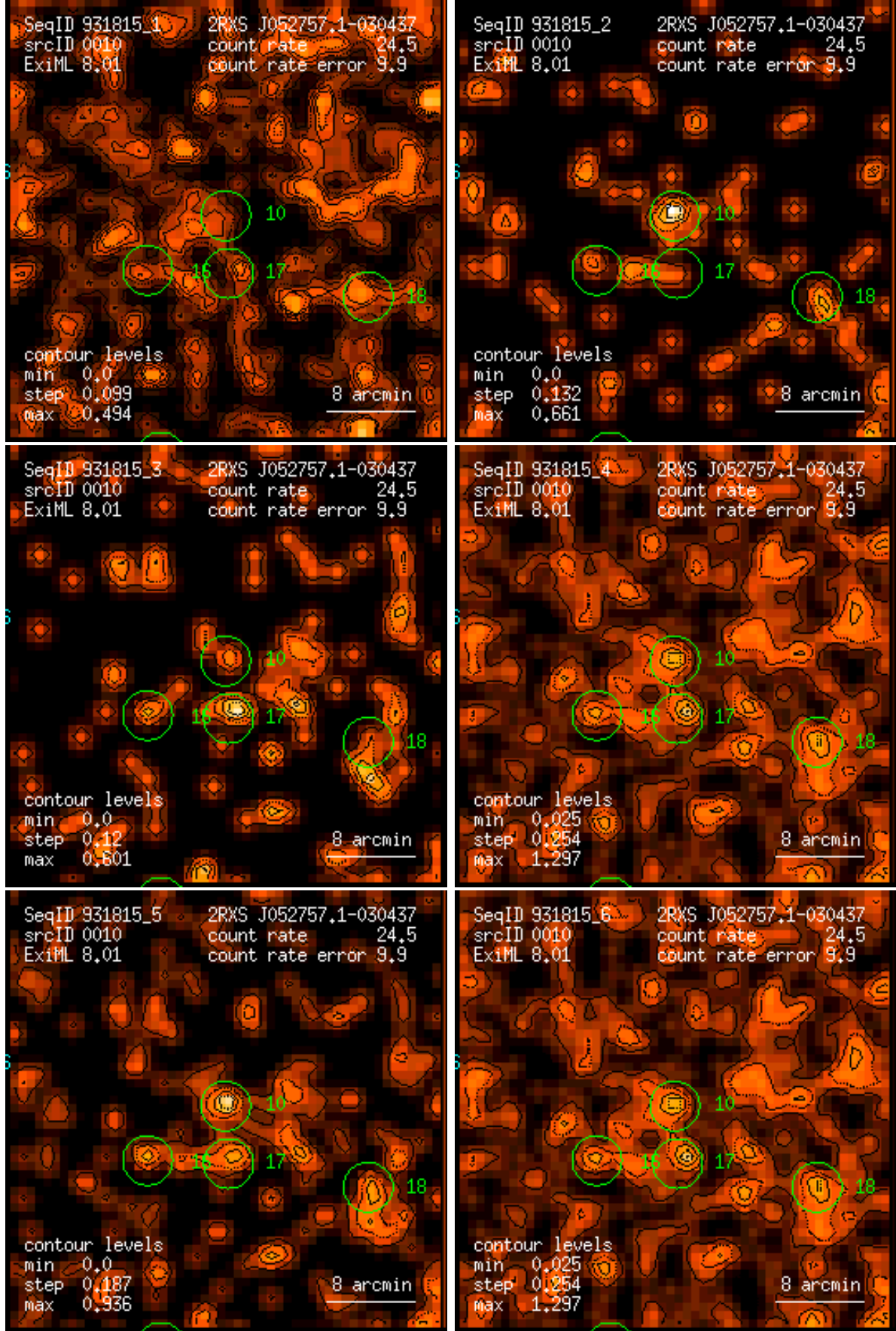
Figure 10: RASS 931815: detection 0010: band rate images, Gaussian filter: (1) PSPC channels 11 – 41, (2) 52 – 90, (3) 91 – 201, (4) 11 – 235, (5) 52 – 201, (6) 11 – 201. Broad band rates in counts/ks. Band rate contour levels in counts/ks/arcmin 2 .
