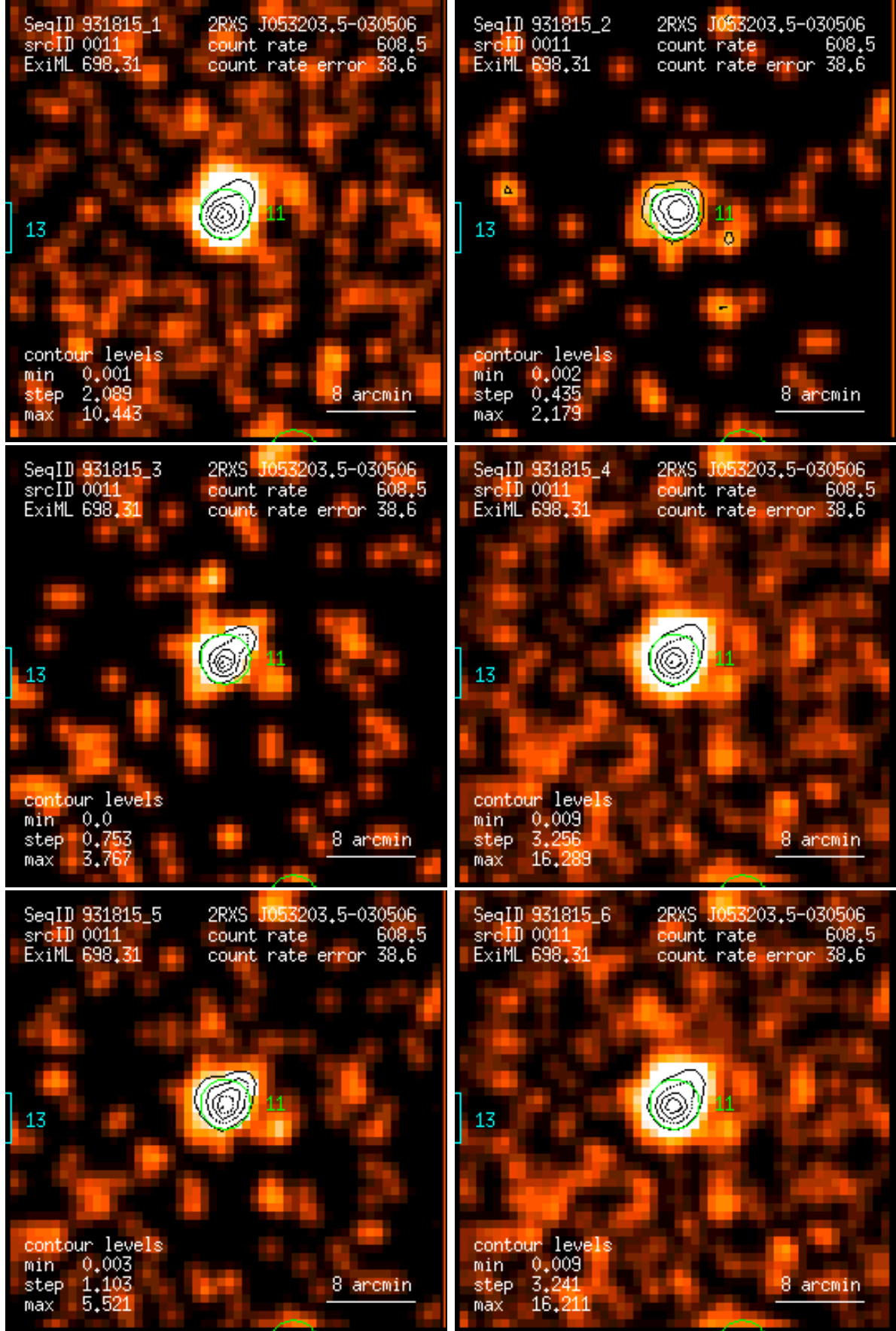
Figure 11: RASS 931815: detection 0011: band rate images, Gaussian filter: (1) PSPC channels 11 – 41, (2) 52 – 90, (3) 91 – 201, (4) 11 – 235, (5) 52 – 201, (6) 11 – 201. Broad band rates in counts/ks. Band rate contour levels in counts/ks/arcmin 2 .
