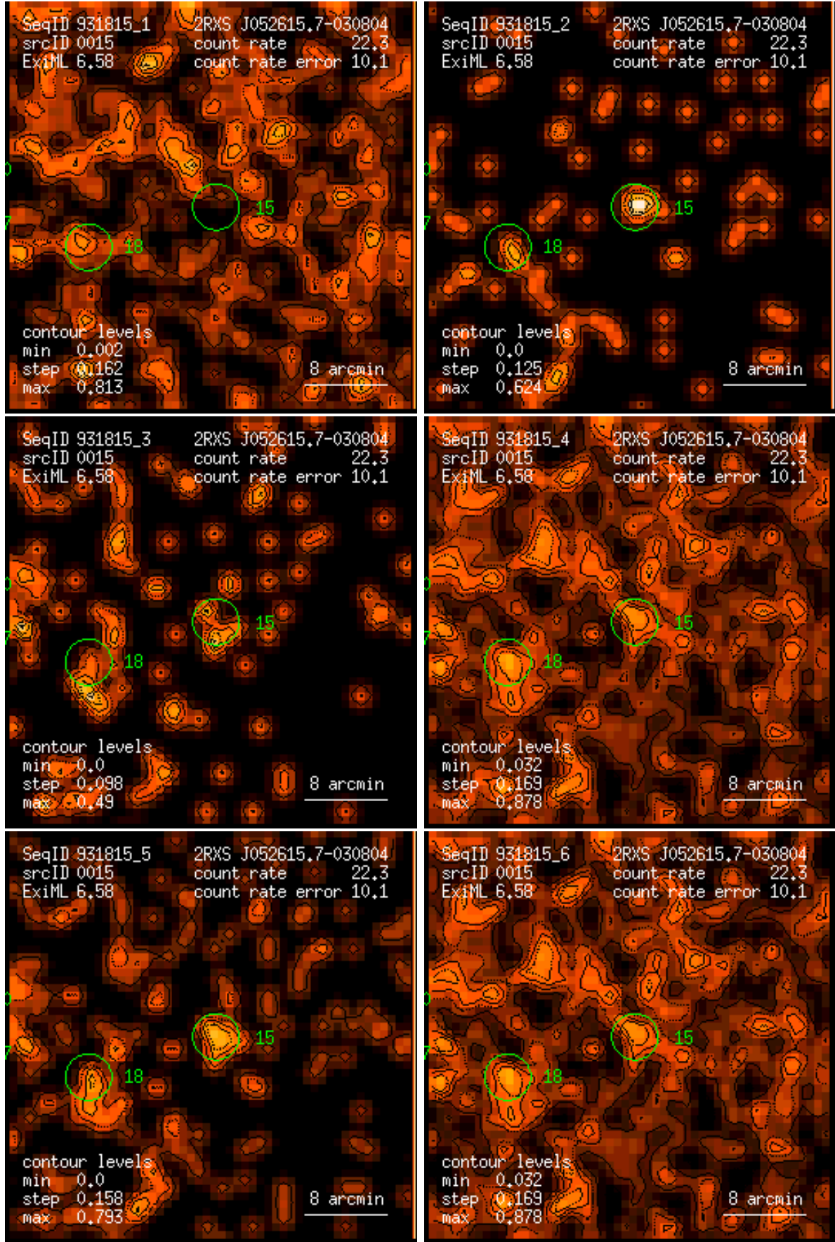
Figure 15: RASS 931815: detection 0015: band rate images, Gaussian filter: (1) PSPC channels 11 – 41, (2) 52 – 90, (3) 91 – 201, (4) 11 – 235, (5) 52 – 201, (6) 11 – 201. Broad band rates in counts/ks. Band rate contour levels in counts/ks/arcmin 2 .
