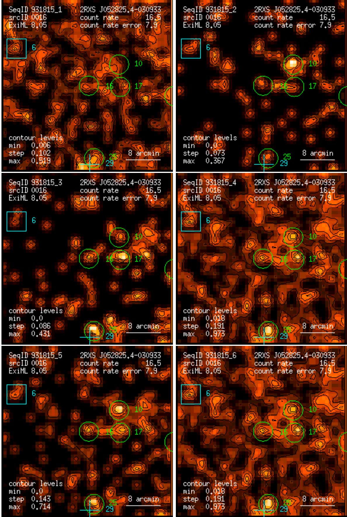
Figure 16: RASS 931815: detection 0016: band rate images, Gaussian filter: (1) PSPC channels 11 – 41, (2) 52 – 90, (3) 91 – 201, (4) 11 – 235, (5) 52 – 201, (6) 11 – 201. Broad band rates in counts/ks. Band rate contour levels in counts/ks/arcmin 2 .
