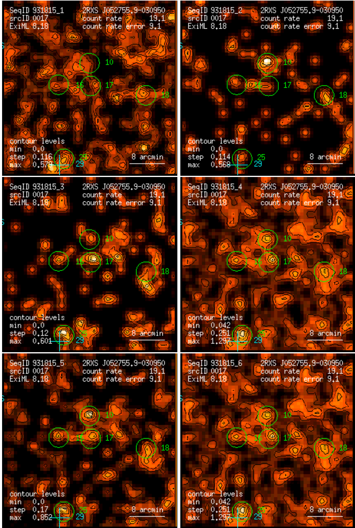
Figure 17: RASS 931815: detection 0017: band rate images, Gaussian filter: (1) PSPC channels 11 – 41, (2) 52 – 90, (3) 91 – 201, (4) 11 – 235, (5) 52 – 201, (6) 11 – 201. Broad band rates in counts/ks. Band rate contour levels in counts/ks/arcmin 2 .
