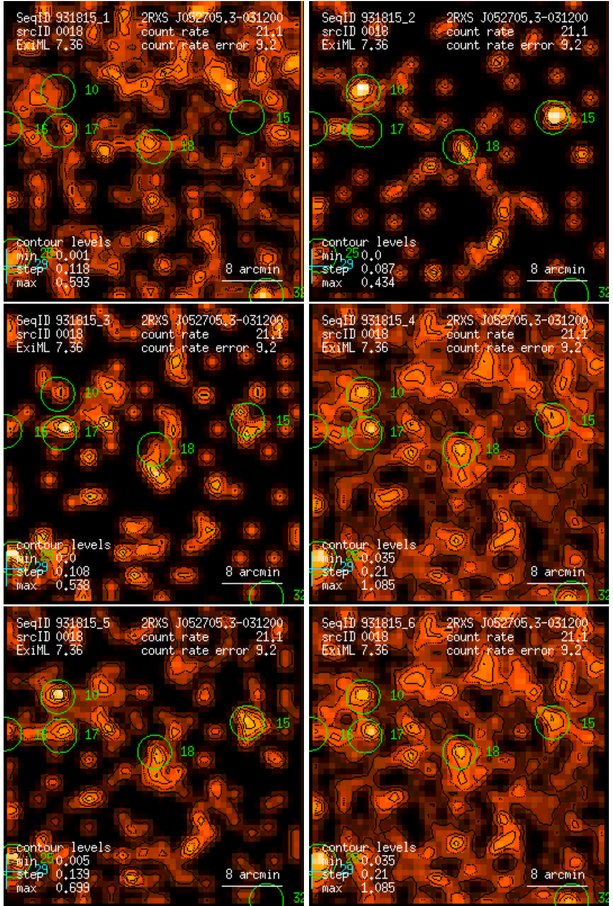
Figure 18: RASS 931815: detection 0018: band rate images, Gaussian filter: (1) PSPC channels 11 – 41, (2) 52 – 90, (3) 91 – 201, (4) 11 – 235, (5) 52 – 201, (6) 11 – 201. Broad band rates in counts/ks. Band rate contour levels in counts/ks/arcmin 2 .
