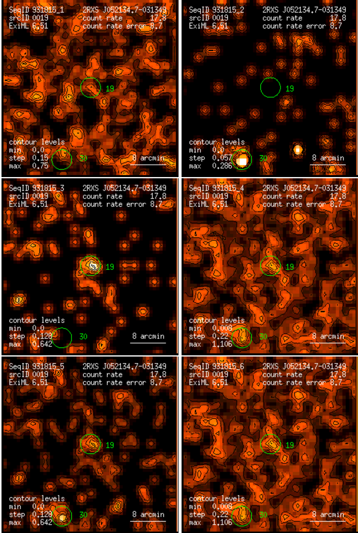
Figure 19: RASS 931815: detection 0019: band rate images, Gaussian filter: (1) PSPC channels 11 – 41, (2) 52 – 90, (3) 91 – 201, (4) 11 – 235, (5) 52 – 201, (6) 11 – 201. Broad band rates in counts/ks. Band rate contour levels in counts/ks/arcmin 2 .
