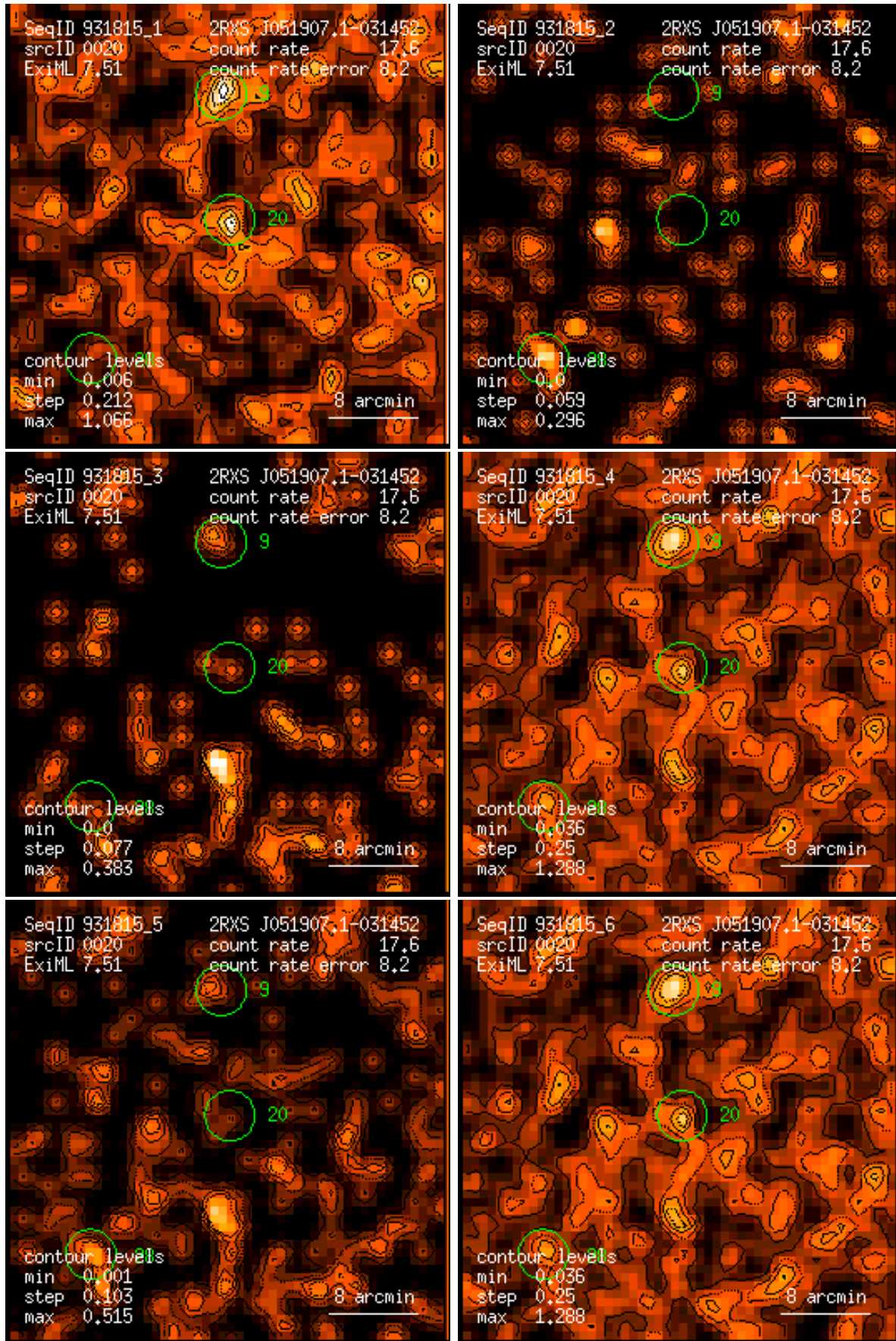
Figure 20: RASS 931815: detection 0020: band rate images, Gaussian filter: (1) PSPC channels 11 – 41, (2) 52 – 90, (3) 91 – 201, (4) 11 – 235, (5) 52 – 201, (6) 11 – 201. Broad band rates in counts/ks. Band rate contour levels in counts/ks/arcmin 2 .
