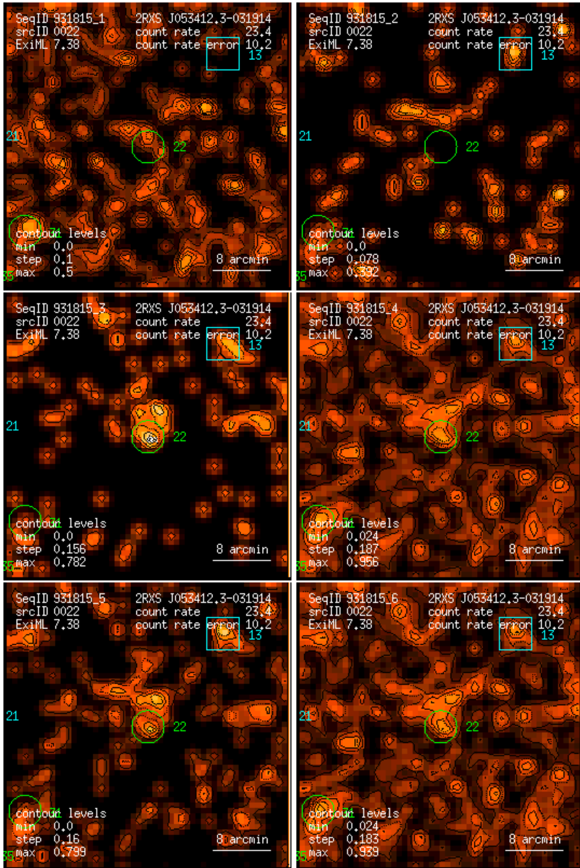
Figure 22: RASS 931815: detection 0022: band rate images, Gaussian filter: (1) PSPC channels 11 – 41, (2) 52 – 90, (3) 91 – 201, (4) 11 – 235, (5) 52 – 201, (6) 11 – 201. Broad band rates in counts/ks. Band rate contour levels in counts/ks/arcmin 2 .
