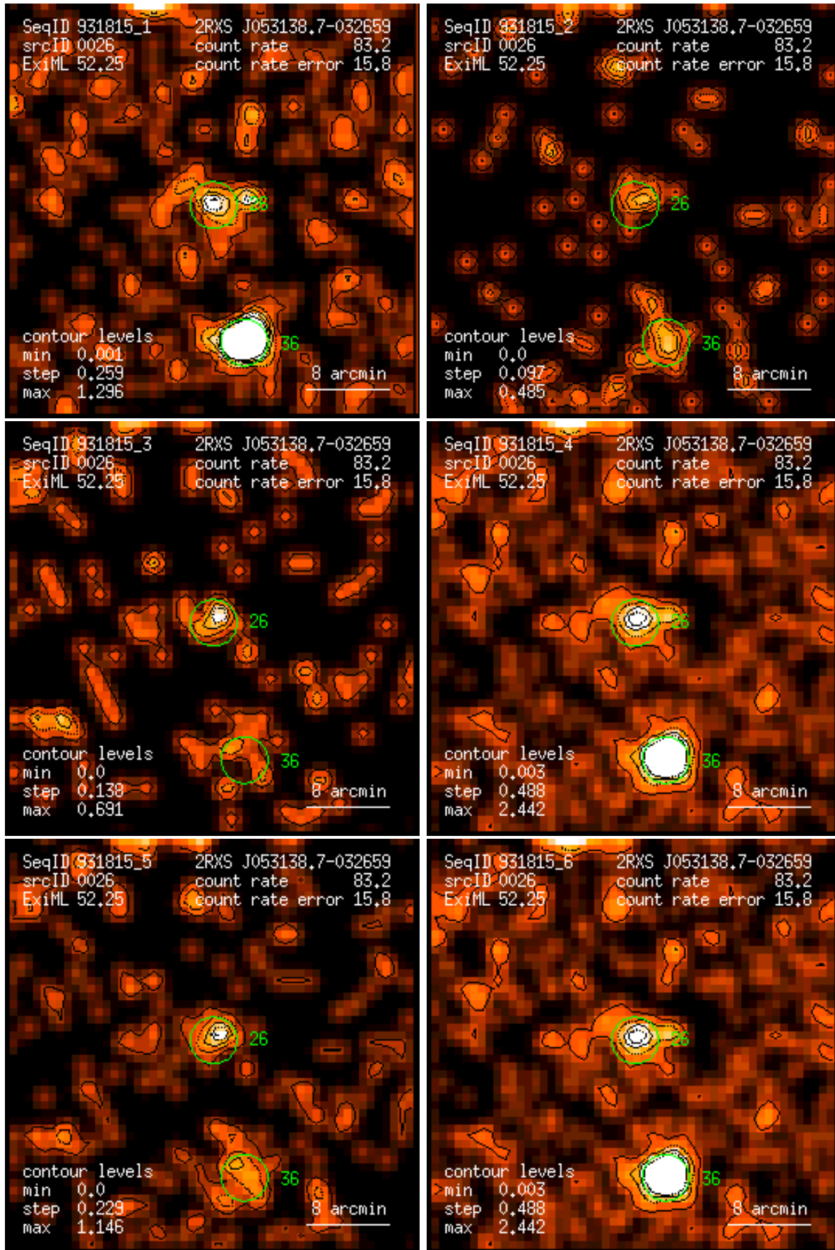
Figure 26: RASS 931815: detection 0026: band rate images, Gaussian filter: (1) PSPC channels 11 – 41, (2) 52 – 90, (3) 91 – 201, (4) 11 – 235, (5) 52 – 201, (6) 11 – 201. Broad band rates in counts/ks. Band rate contour levels in counts/ks/arcmin 2 .
