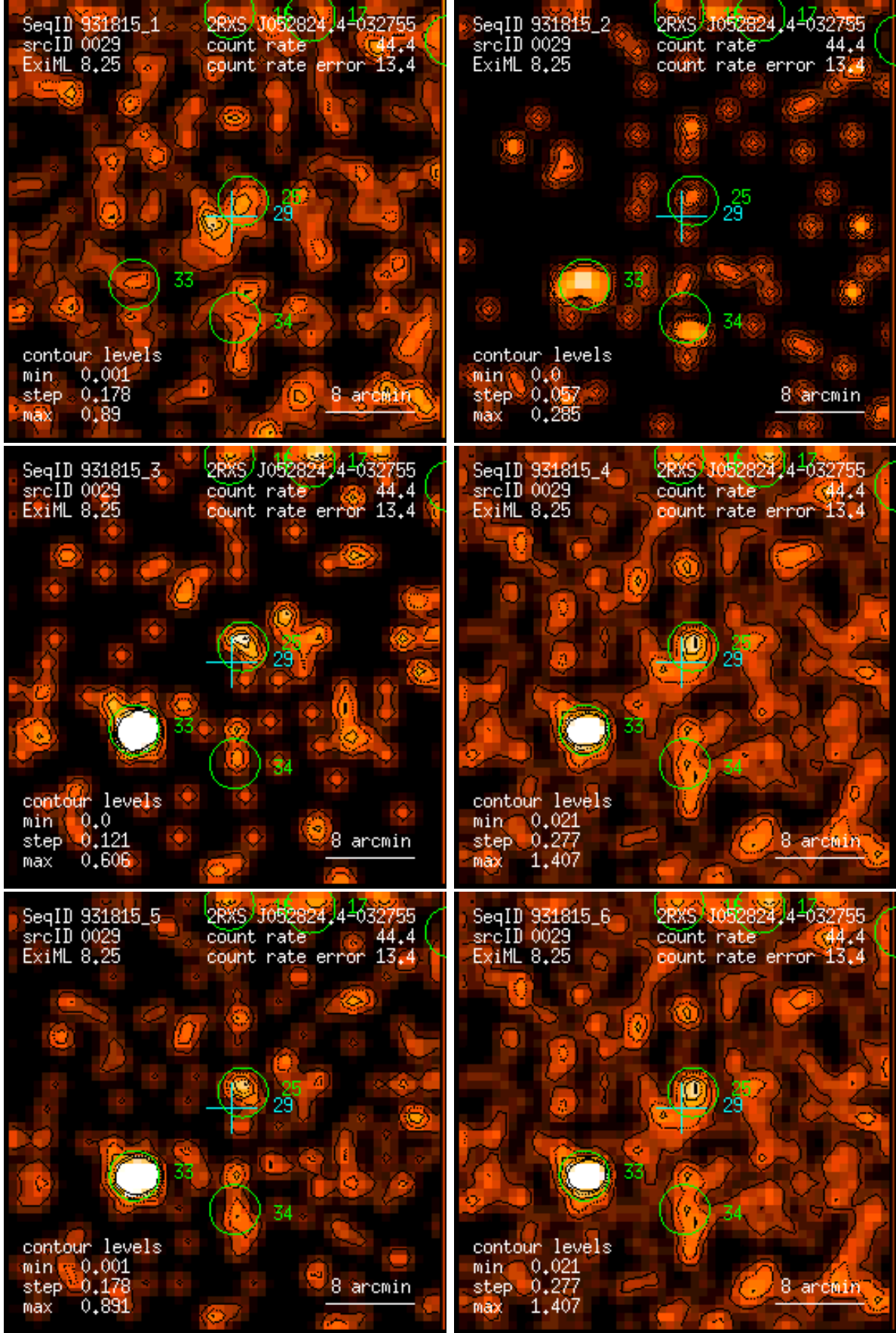
Figure 29: RASS 931815: detection 0029: band rate images, Gaussian filter: (1) PSPC channels 11 – 41, (2) 52 – 90, (3) 91 – 201, (4) 11 – 235, (5) 52 – 201, (6) 11 – 201. Broad band rates in counts/ks. Band rate contour levels in counts/ks/arcmin 2 .
