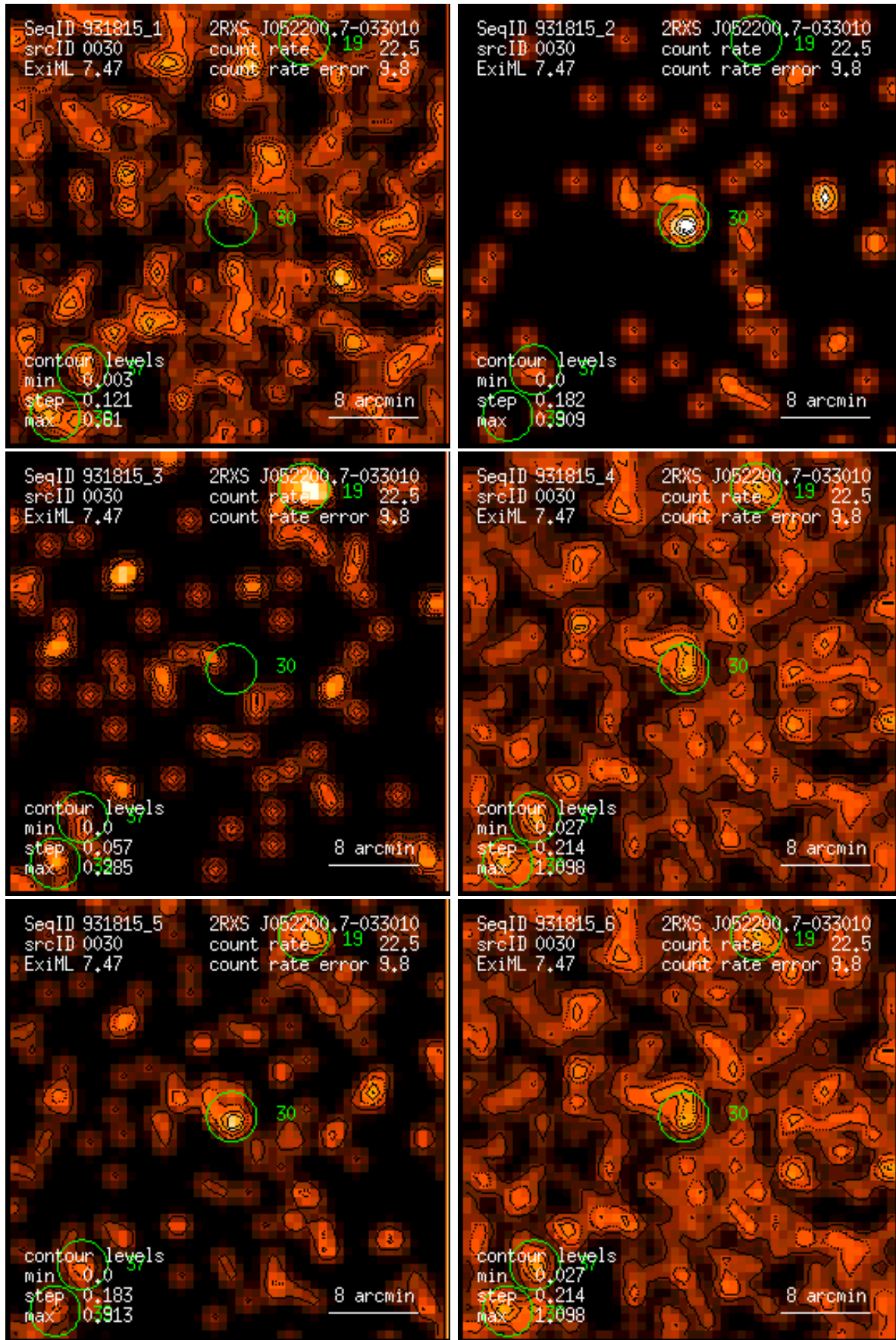
Figure 30: RASS 931815: detection 0030: band rate images, Gaussian filter: (1) PSPC channels 11 – 41, (2) 52 – 90, (3) 91 – 201, (4) 11 – 235, (5) 52 – 201, (6) 11 – 201. Broad band rates in counts/ks. Band rate contour levels in counts/ks/arcmin 2 .
