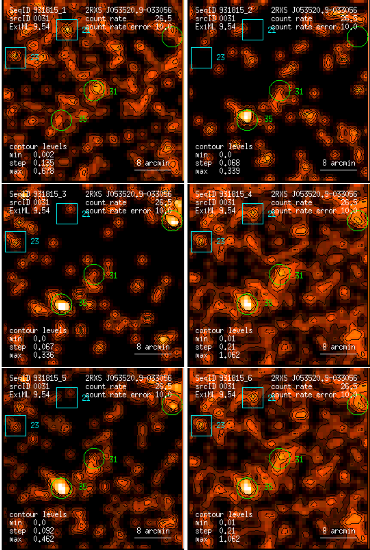
Figure 31: RASS 931815: detection 0031: band rate images, Gaussian filter: (1) PSPC channels 11 – 41, (2) 52 – 90, (3) 91 – 201, (4) 11 – 235, (5) 52 – 201, (6) 11 – 201. Broad band rates in counts/ks. Band rate contour levels in counts/ks/arcmin 2 .
