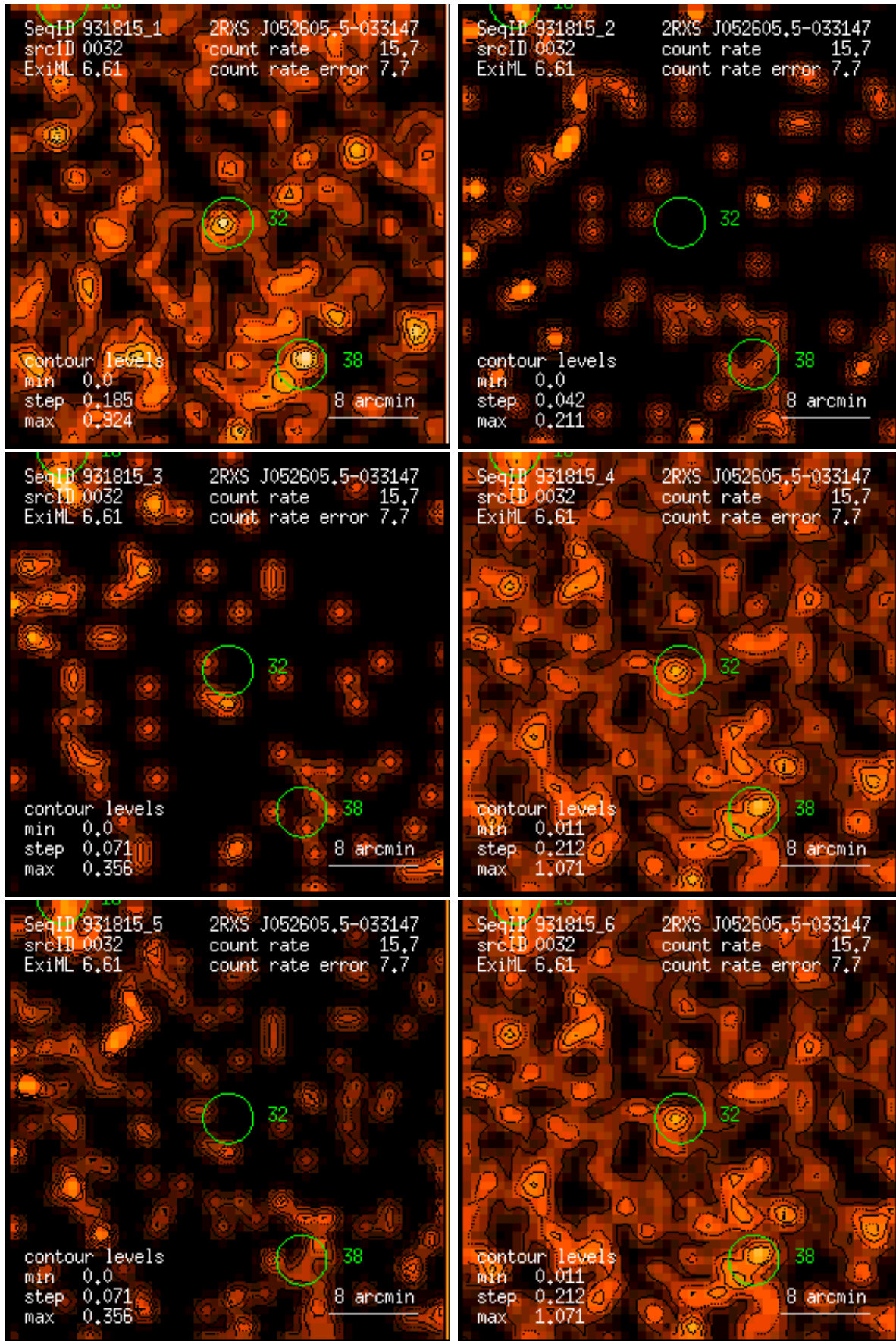
Figure 32: RASS 931815: detection 0032: band rate images, Gaussian filter: (1) PSPC channels 11 – 41, (2) 52 – 90, (3) 91 – 201, (4) 11 – 235, (5) 52 – 201, (6) 11 – 201. Broad band rates in counts/ks. Band rate contour levels in counts/ks/arcmin 2 .
