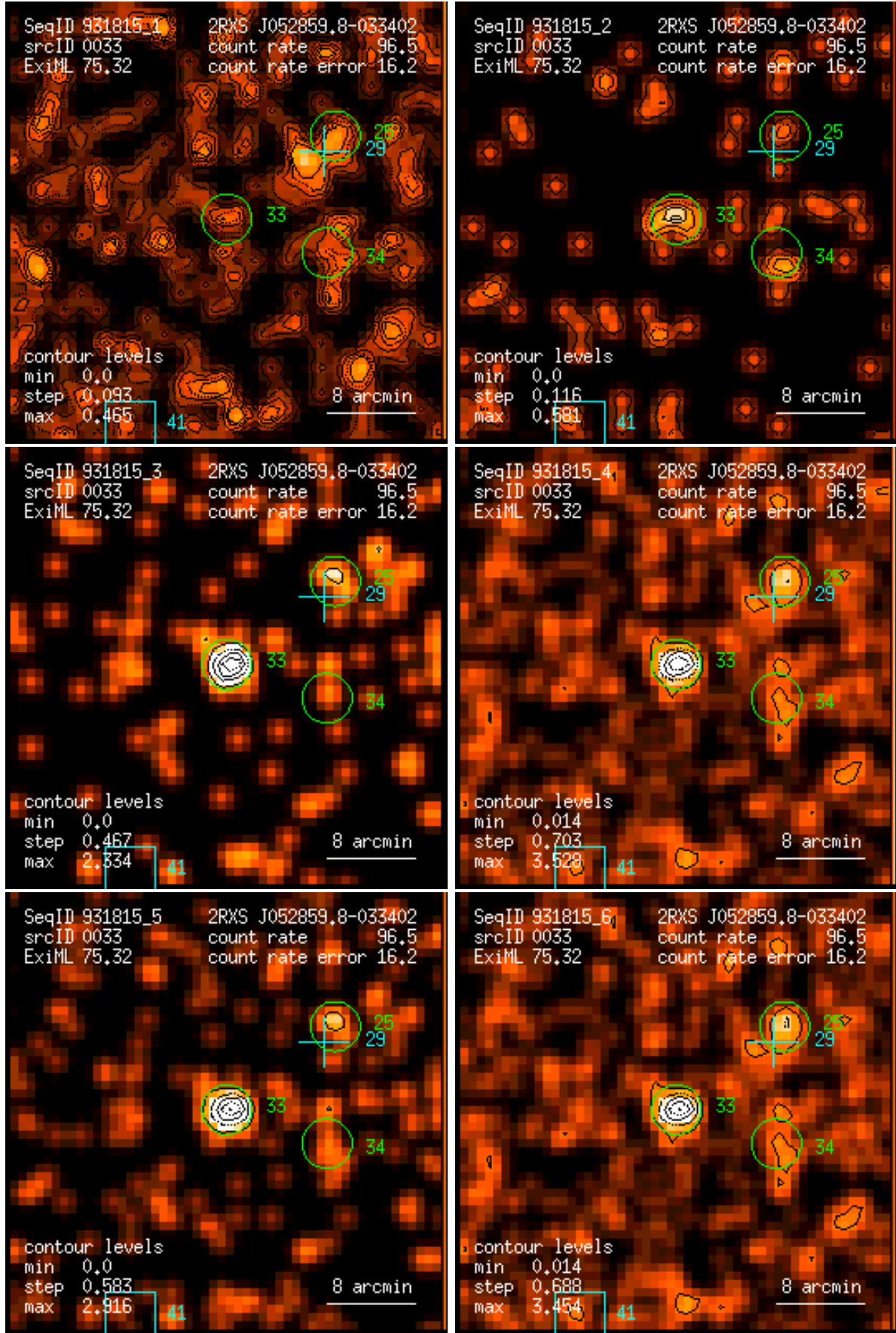
Figure 33: RASS 931815: detection 0033: band rate images, Gaussian filter: (1) PSPC channels 11 – 41, (2) 52 – 90, (3) 91 – 201, (4) 11 – 235, (5) 52 – 201, (6) 11 – 201. Broad band rates in counts/ks. Band rate contour levels in counts/ks/arcmin 2 .
