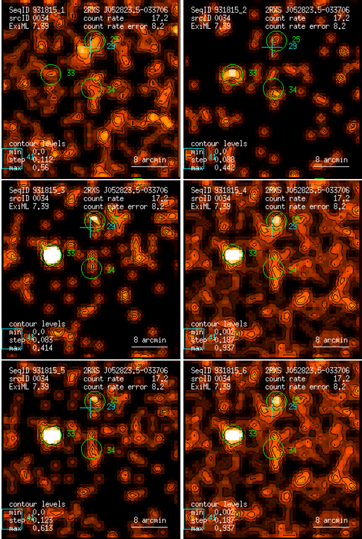
Figure 34: RASS 931815: detection 0034: band rate images, Gaussian filter: (1) PSPC channels 11 – 41, (2) 52 – 90, (3) 91 – 201, (4) 11 – 235, (5) 52 – 201, (6) 11 – 201. Broad band rates in counts/ks. Band rate contour levels in counts/ks/arcmin 2 .
