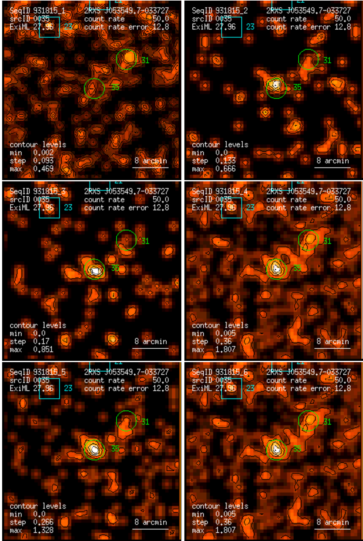
Figure 35: RASS 931815: detection 0035: band rate images, Gaussian filter: (1) PSPC channels 11 – 41, (2) 52 – 90, (3) 91 – 201, (4) 11 – 235, (5) 52 – 201, (6) 11 – 201. Broad band rates in counts/ks. Band rate contour levels in counts/ks/arcmin 2 .
