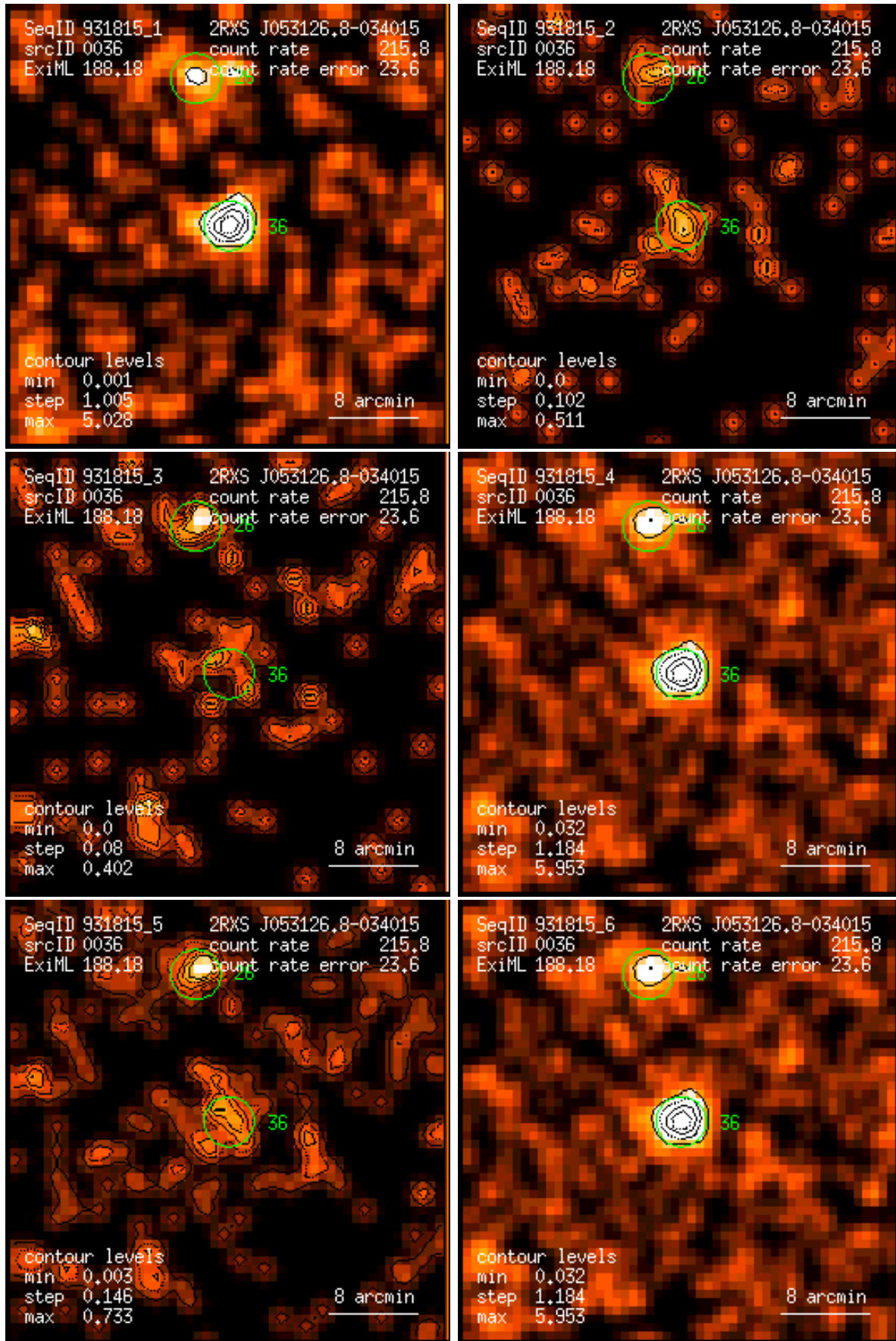
Figure 36: RASS 931815: detection 0036: band rate images, Gaussian filter: (1) PSPC channels 11 – 41, (2) 52 – 90, (3) 91 – 201, (4) 11 – 235, (5) 52 – 201, (6) 11 – 201. Broad band rates in counts/ks. Band rate contour levels in counts/ks/arcmin 2 .
