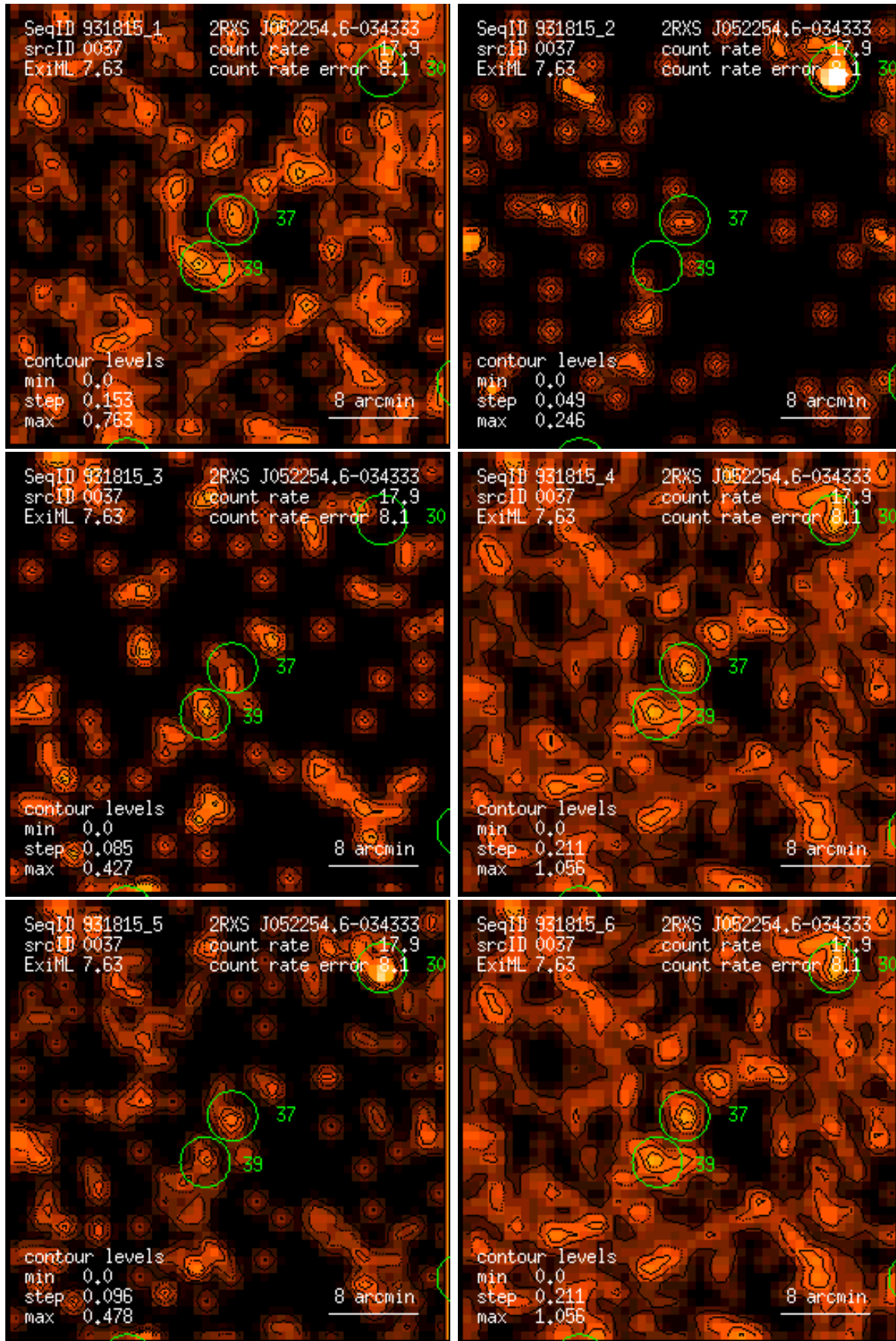
Figure 37: RASS 931815: detection 0037: band rate images, Gaussian filter: (1) PSPC channels 11 – 41, (2) 52 – 90, (3) 91 – 201, (4) 11 – 235, (5) 52 – 201, (6) 11 – 201. Broad band rates in counts/ks. Band rate contour levels in counts/ks/arcmin 2 .
