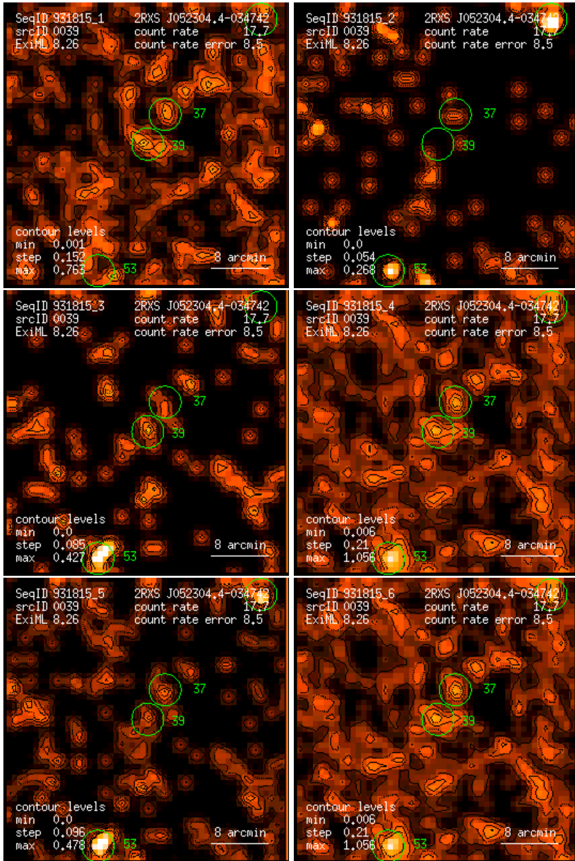
Figure 39: RASS 931815: detection 0039: band rate images, Gaussian filter: (1) PSPC channels 11 – 41, (2) 52 – 90, (3) 91 – 201, (4) 11 – 235, (5) 52 – 201, (6) 11 – 201. Broad band rates in counts/ks. Band rate contour levels in counts/ks/arcmin 2 .
