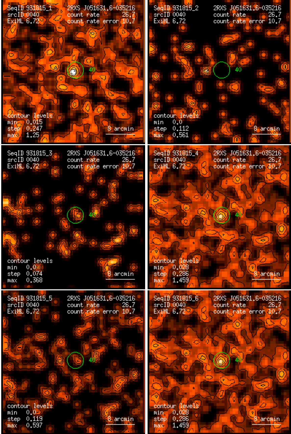
Figure 40: RASS 931815: detection 0040: band rate images, Gaussian filter: (1) PSPC channels 11 – 41, (2) 52 – 90, (3) 91 – 201, (4) 11 – 235, (5) 52 – 201, (6) 11 – 201. Broad band rates in counts/ks. Band rate contour levels in counts/ks/arcmin 2 .
