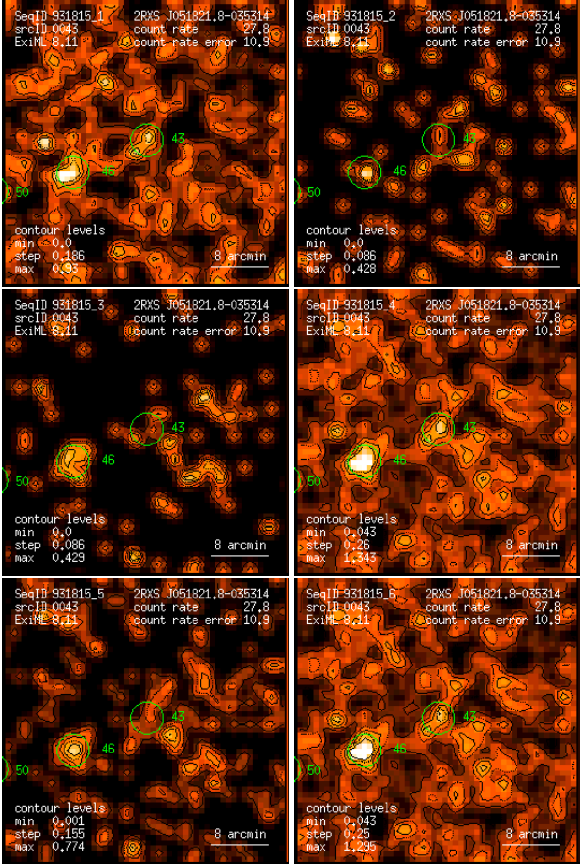
Figure 43: RASS 931815: detection 0043: band rate images, Gaussian filter: (1) PSPC channels 11 – 41, (2) 52 – 90, (3) 91 – 201, (4) 11 – 235, (5) 52 – 201, (6) 11 – 201. Broad band rates in counts/ks. Band rate contour levels in counts/ks/arcmin 2 .
