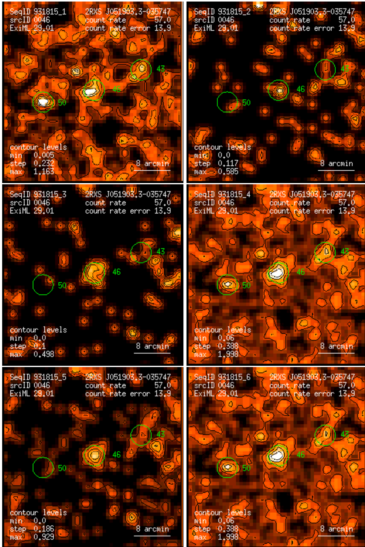
Figure 46: RASS 931815: detection 0046: band rate images, Gaussian filter: (1) PSPC channels 11 – 41, (2) 52 – 90, (3) 91 – 201, (4) 11 – 235, (5) 52 – 201, (6) 11 – 201. Broad band rates in counts/ks. Band rate contour levels in counts/ks/arcmin 2 .
