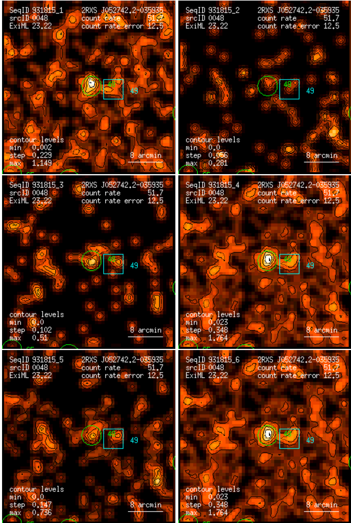
Figure 48: RASS 931815: detection 0048: band rate images, Gaussian filter: (1) PSPC channels 11 – 41, (2) 52 – 90, (3) 91 – 201, (4) 11 – 235, (5) 52 – 201, (6) 11 – 201. Broad band rates in counts/ks. Band rate contour levels in counts/ks/arcmin 2 .
