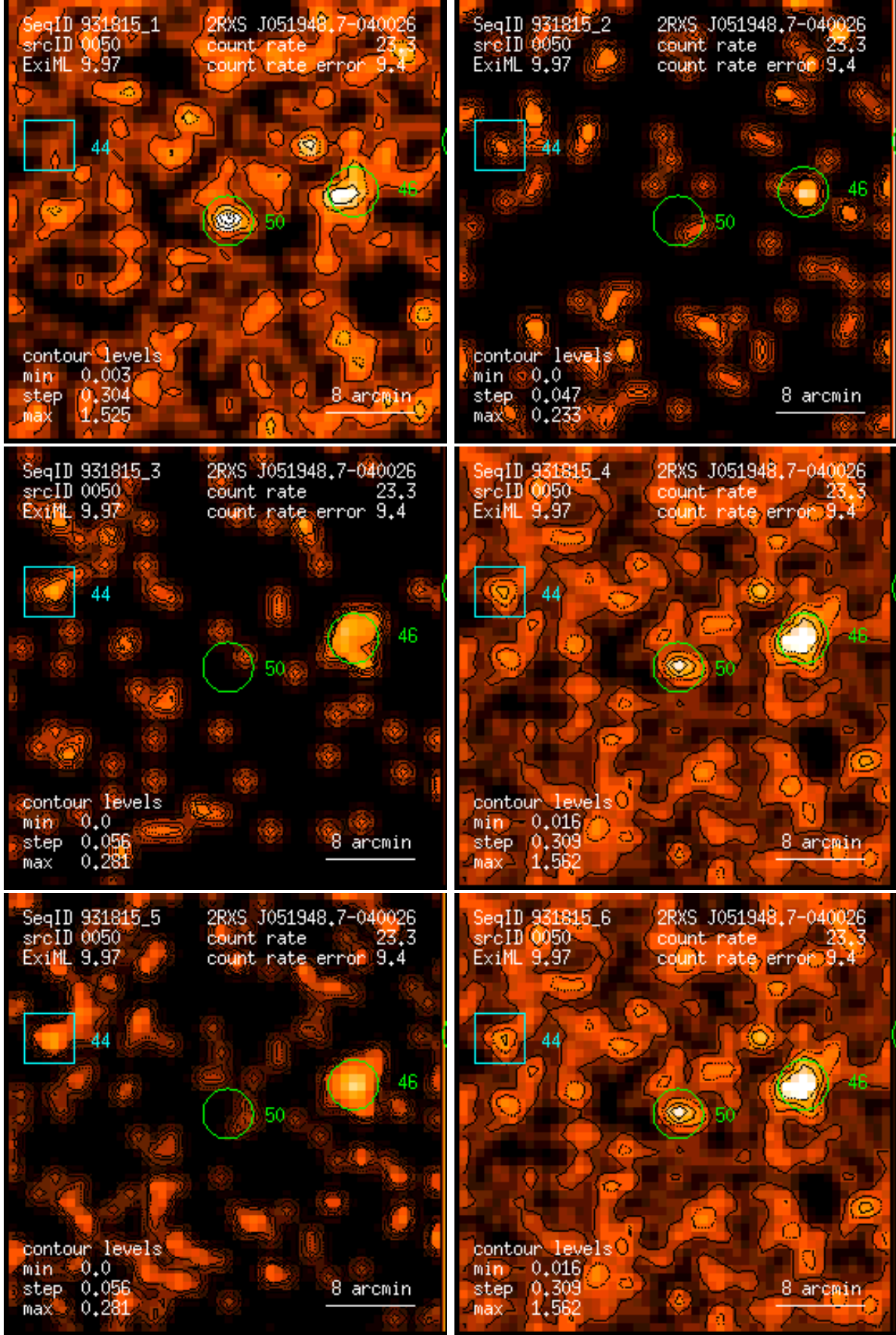
Figure 50: RASS 931815: detection 0050: band rate images, Gaussian filter: (1) PSPC channels 11 – 41, (2) 52 – 90, (3) 91 – 201, (4) 11 – 235, (5) 52 – 201, (6) 11 – 201. Broad band rates in counts/ks. Band rate contour levels in counts/ks/arcmin 2 .
