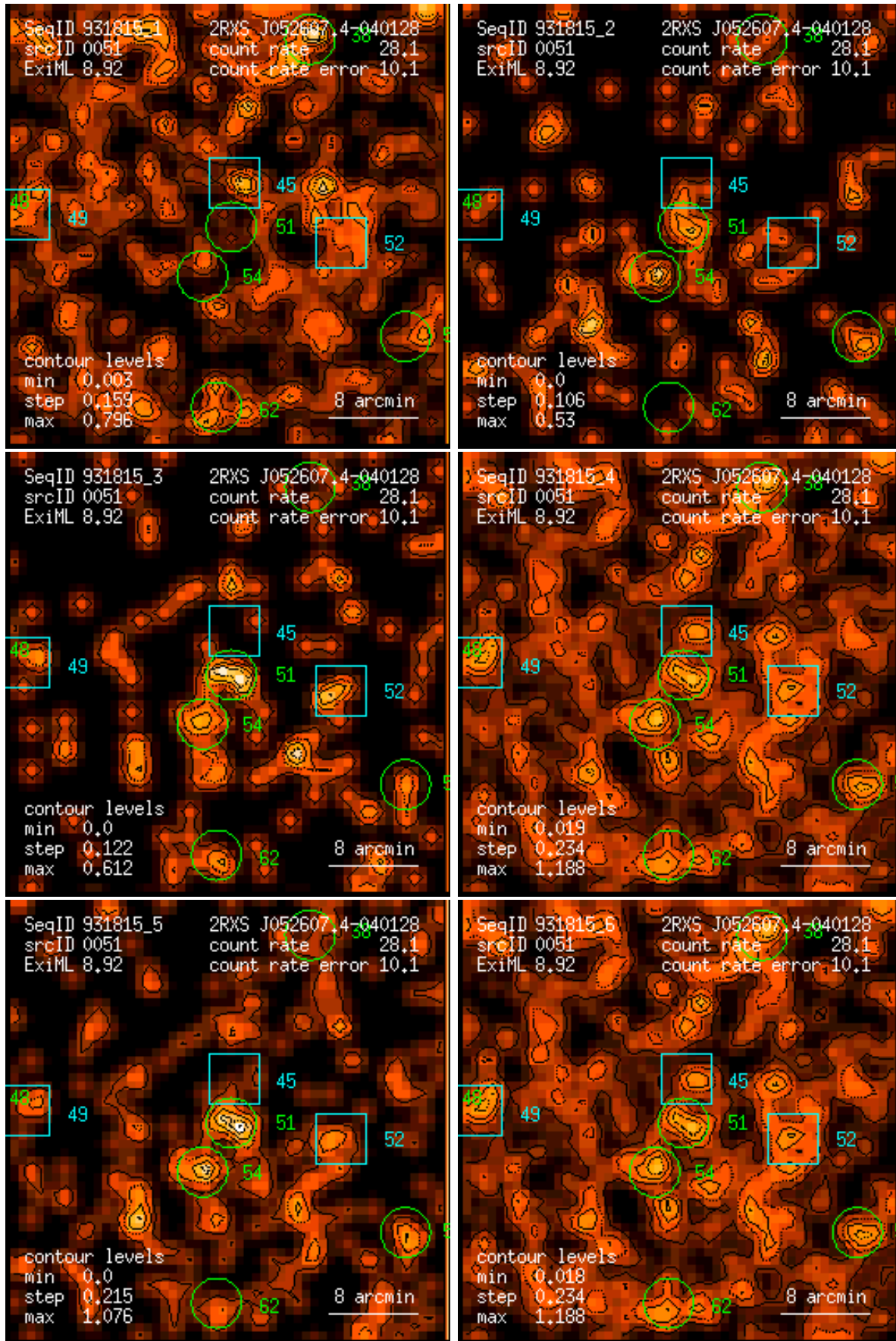
Figure 51: RASS 931815: detection 0051: band rate images, Gaussian filter: (1) PSPC channels 11 – 41, (2) 52 – 90, (3) 91 – 201, (4) 11 – 235, (5) 52 – 201, (6) 11 – 201. Broad band rates in counts/ks. Band rate contour levels in counts/ks/arcmin 2 .
