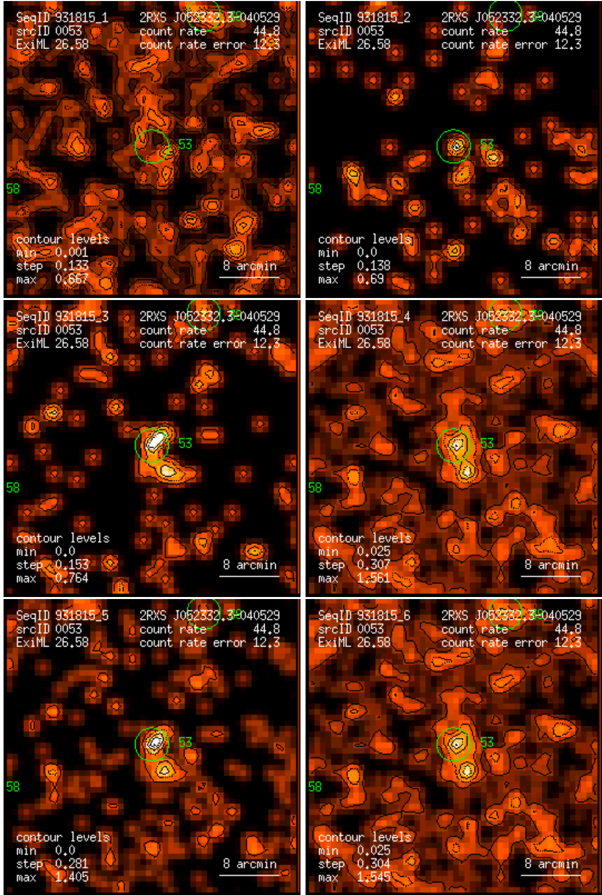
Figure 53: RASS 931815: detection 0053: band rate images, Gaussian filter: (1) PSPC channels 11 – 41, (2) 52 – 90, (3) 91 – 201, (4) 11 – 235, (5) 52 – 201, (6) 11 – 201. Broad band rates in counts/ks. Band rate contour levels in counts/ks/arcmin 2 .
