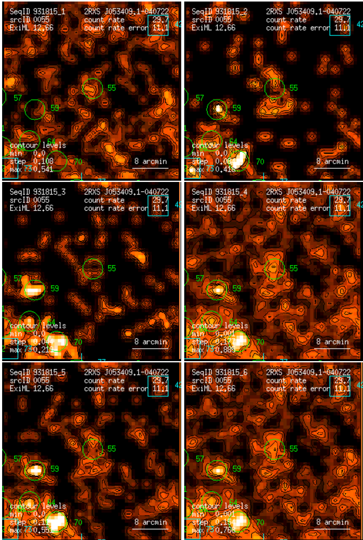
Figure 55: RASS 931815: detection 0055: band rate images, Gaussian filter: (1) PSPC channels 11 – 41, (2) 52 – 90, (3) 91 – 201, (4) 11 – 235, (5) 52 – 201, (6) 11 – 201. Broad band rates in counts/ks. Band rate contour levels in counts/ks/arcmin 2 .
