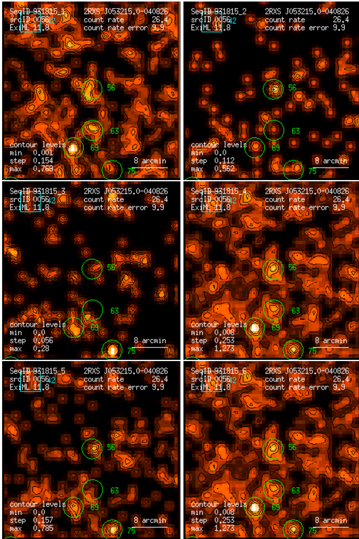
Figure 56: RASS 931815: detection 0056: band rate images, Gaussian filter: (1) PSPC channels 11 – 41, (2) 52 – 90, (3) 91 – 201, (4) 11 – 235, (5) 52 – 201, (6) 11 – 201. Broad band rates in counts/ks. Band rate contour levels in counts/ks/arcmin 2 .
