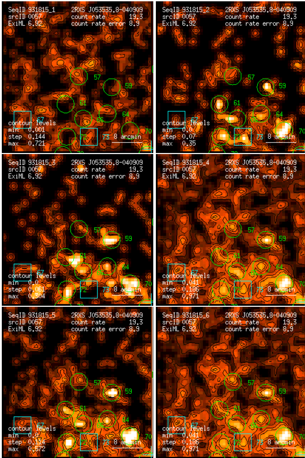
Figure 57: RASS 931815: detection 0057: band rate images, Gaussian filter: (1) PSPC channels 11 – 41, (2) 52 – 90, (3) 91 – 201, (4) 11 – 235, (5) 52 – 201, (6) 11 – 201. Broad band rates in counts/ks. Band rate contour levels in counts/ks/arcmin 2 .
