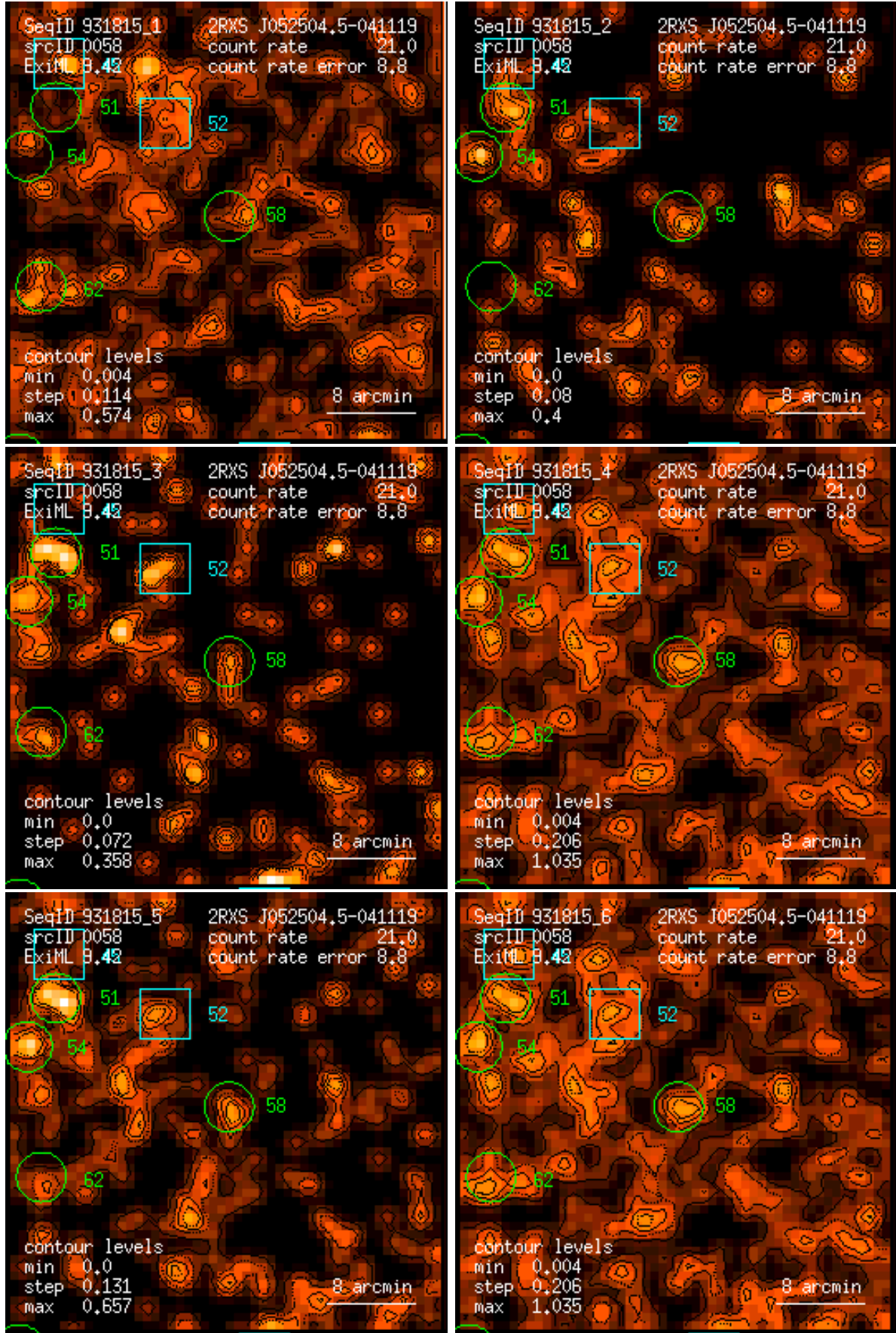
Figure 58: RASS 931815: detection 0058: band rate images, Gaussian filter: (1) PSPC channels 11 – 41, (2) 52 – 90, (3) 91 – 201, (4) 11 – 235, (5) 52 – 201, (6) 11 – 201. Broad band rates in counts/ks. Band rate contour levels in counts/ks/arcmin 2 .
