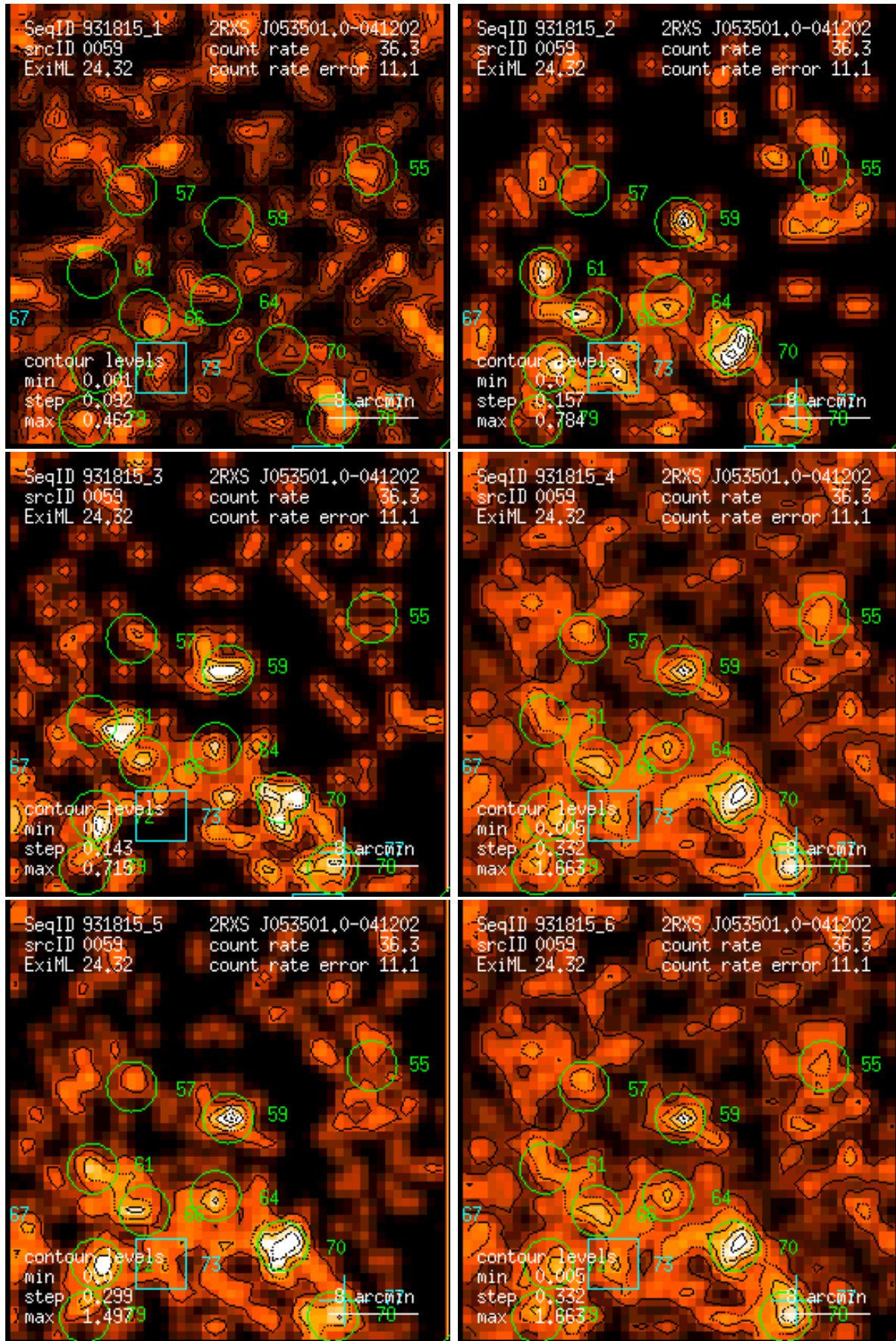
Figure 59: RASS 931815: detection 0059: band rate images, Gaussian filter: (1) PSPC channels 11 – 41, (2) 52 – 90, (3) 91 – 201, (4) 11 – 235, (5) 52 – 201, (6) 11 – 201. Broad band rates in counts/ks. Band rate contour levels in counts/ks/arcmin 2 .
