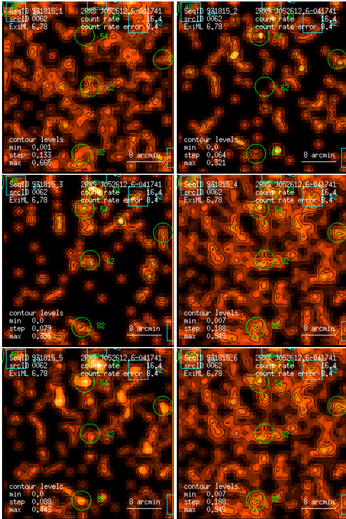
Figure 62: RASS 931815: detection 0062: band rate images, Gaussian filter: (1) PSPC channels 11 – 41, (2) 52 – 90, (3) 91 – 201, (4) 11 – 235, (5) 52 – 201, (6) 11 – 201. Broad band rates in counts/ks. Band rate contour levels in counts/ks/arcmin 2 .
