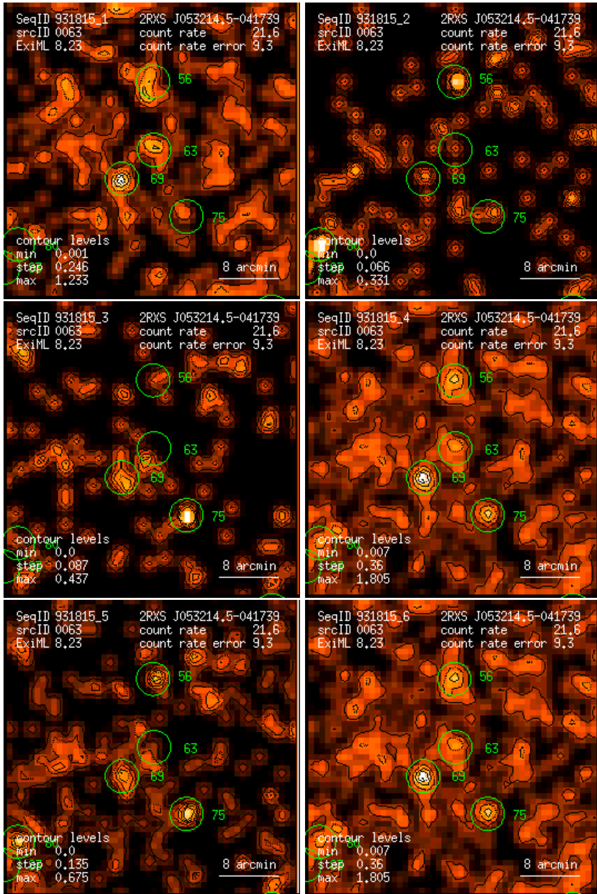
Figure 63: RASS 931815: detection 0063: band rate images, Gaussian filter: (1) PSPC channels 11 – 41, (2) 52 – 90, (3) 91 – 201, (4) 11 – 235, (5) 52 – 201, (6) 11 – 201. Broad band rates in counts/ks. Band rate contour levels in counts/ks/arcmin 2 .
