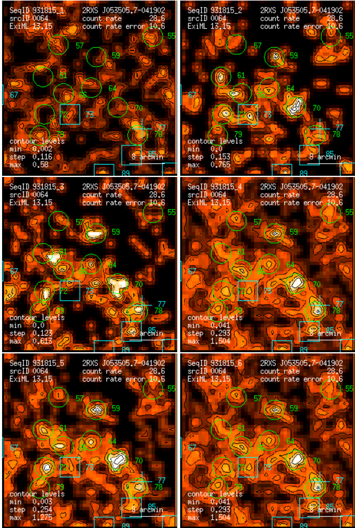
Figure 64: RASS 931815: detection 0064: band rate images, Gaussian filter: (1) PSPC channels 11 – 41, (2) 52 – 90, (3) 91 – 201, (4) 11 – 235, (5) 52 – 201, (6) 11 – 201. Broad band rates in counts/ks. Band rate contour levels in counts/ks/arcmin 2 .
